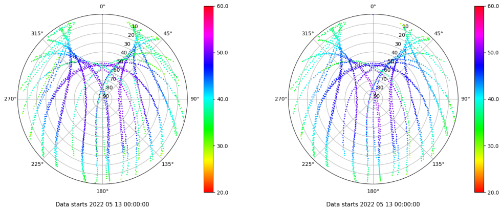
Skyplot for station SEV1. Signal to Noise S1C Data file SEV100ESP_R_2022133.xtr Skyplot for station SEV1. Signal to Noise S2C Data file SEV100ESP_R_2022133.xtr
