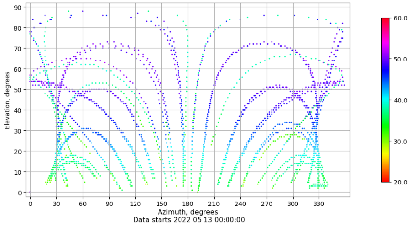
Azimuth-elevation plot for station SEV1. Signal to Noise S1C Data file SEV100ESP_R_2022133.xtr
