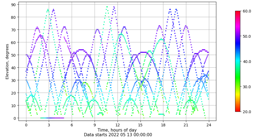
Time-elevation plot for station SEV1. Signal to Noise S1C Data file SEV100ESP_R_2022133.xtr
