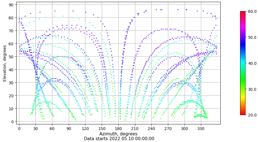
Azimuth-elevation plot for station SEV1. Signal to Noise S1C Data file SEV100ESP_R_2022130.xtr
