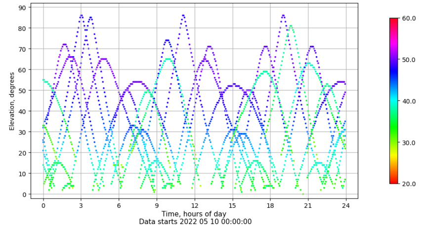
Time-elevation plot for station SEV1. Signal to Noise S1C Data file SEV100ESP_R_2022130.xtr
