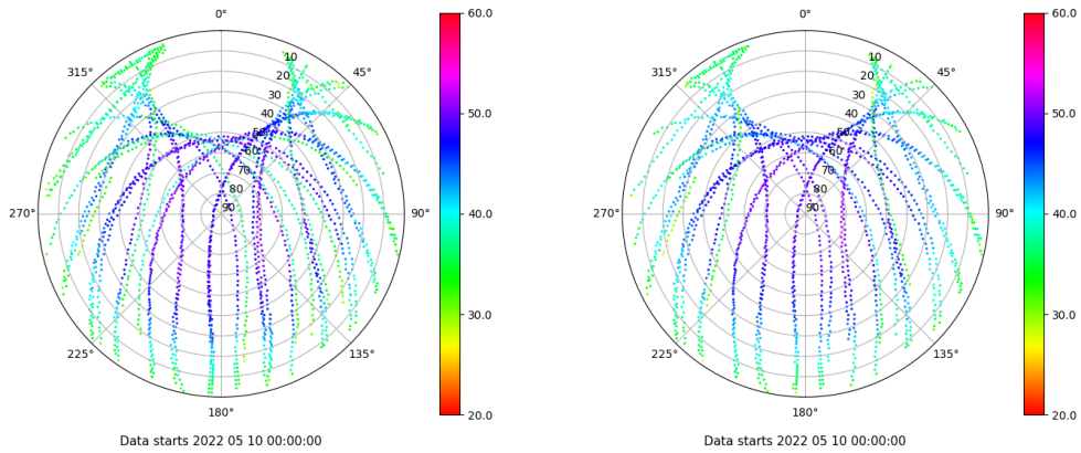
Skyplot for station SEV1. Signal to Noise S1C Data file SEV100ESP_R_2022130.xtr Skyplot for station SEV1. Signal to Noise S2C Data file SEV100ESP_R_2022130.xtr
