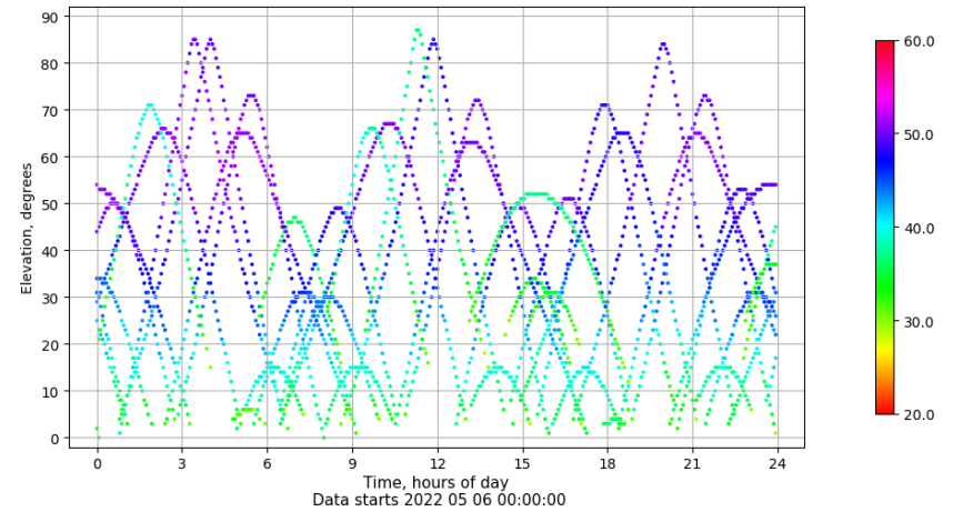
Time-elevation plot for station SEV1. Signal to Noise S1C Data file SEV100ESP_R_2022126.xtr
