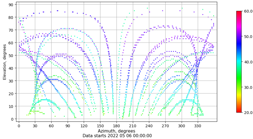
Azimuth-elevation plot for station SEV1. Signal to Noise S1C Data file SEV100ESP_R_2022126.xtr
