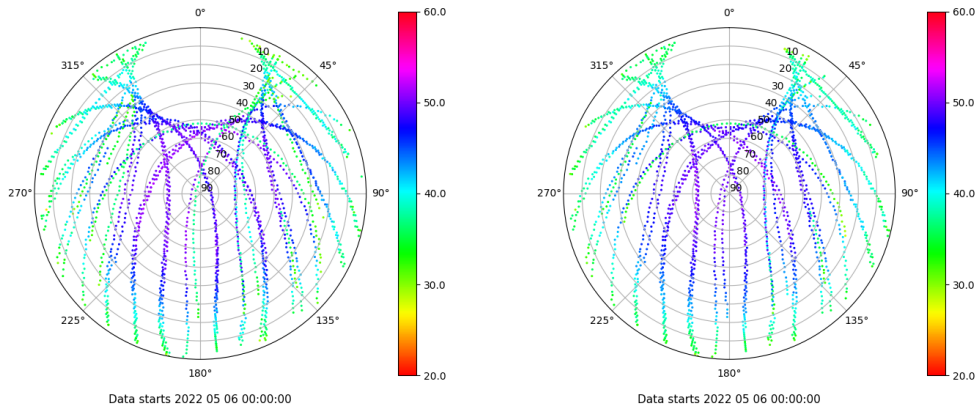
Skyplot for station SEV1. Signal to Noise S1C Data file SEV100ESP_R_2022126.xtr Skyplot for station SEV1. Signal to Noise S2C Data file SEV100ESP_R_2022126.xtr
