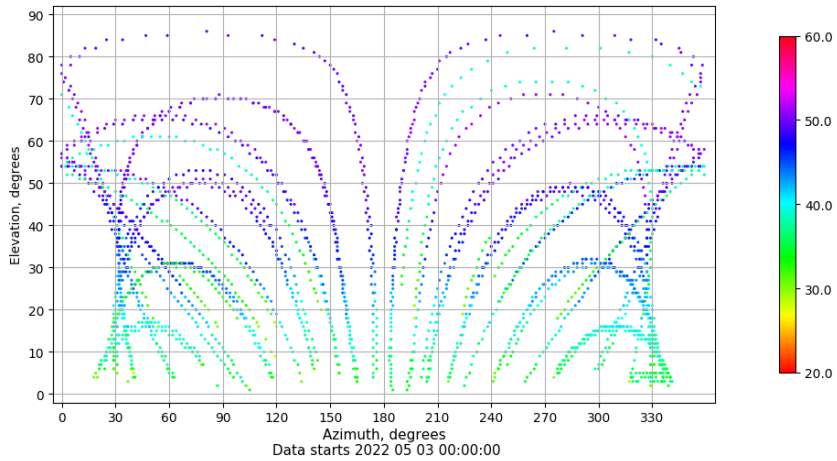
Azimuth-elevation plot for station SEV1. Signal to Noise S1C Data file SEV100ESP_R_2022123.xtr
