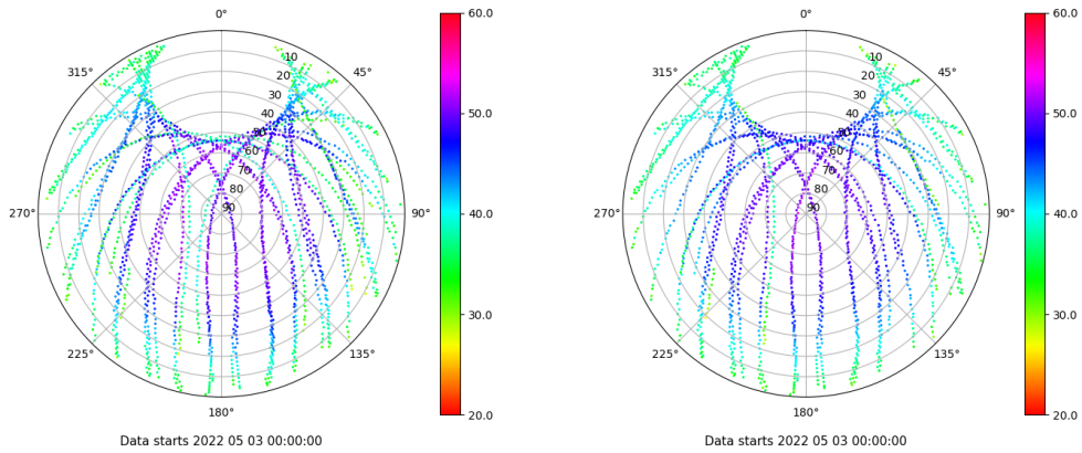
Skyplot for station SEV1. Signal to Noise S1C Data file SEV100ESP_R_2022123.xtr Skyplot for station SEV1. Signal to Noise S2C Data file SEV100ESP_R_2022123.xtr
