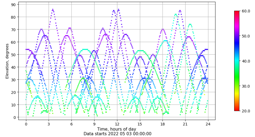
Time-elevation plot for station SEV1. Signal to Noise S1C Data file SEV100ESP_R_2022123.xtr
