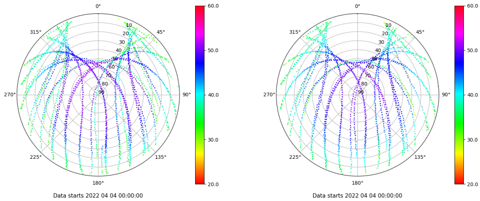
Skyplot for station SEV1. Signal to Noise S1C Data file SEV100ESP_R_2022094.xtr Skyplot for station SEV1. Signal to Noise S2C Data file SEV100ESP_R_2022094.xtr
