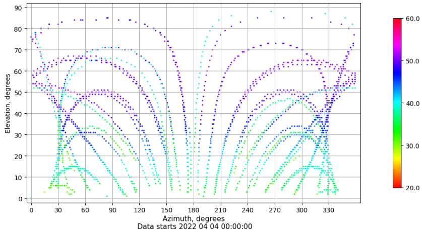
Azimuth-elevation plot for station SEV1. Signal to Noise S1C Data file SEV100ESP_R_2022094.xtr
