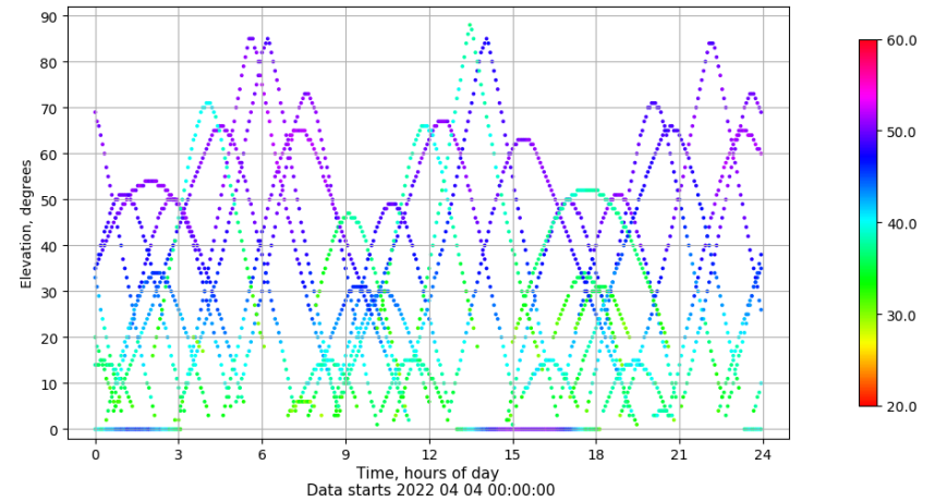
Time-elevation plot for station SEV1. Signal to Noise S1C Data file SEV100ESP_R_2022094.xtr
