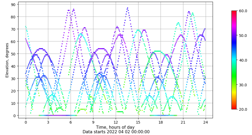
Time-elevation plot for station SEV1. Signal to Noise S1C Data file SEV100ESP_R_2022092.xtr
