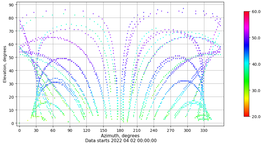
Azimuth-elevation plot for station SEV1. Signal to Noise S1C Data file SEV100ESP_R_2022092.xtr
