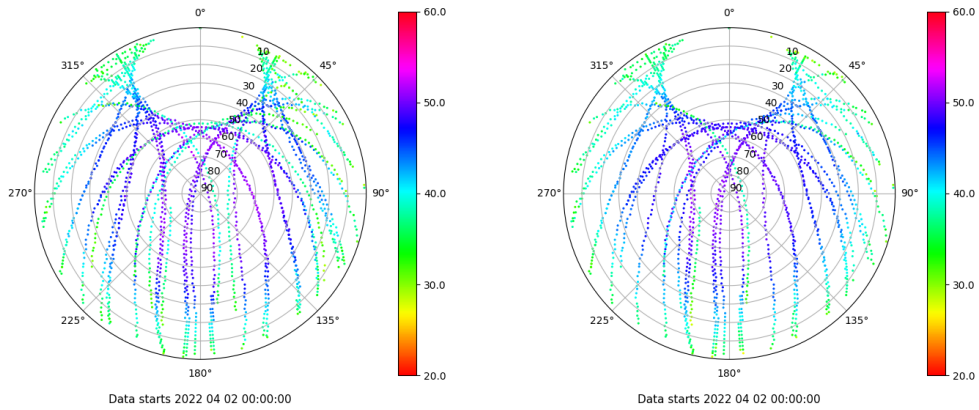
Skyplot for station SEV1. Signal to Noise S1C Data file SEV100ESP_R_2022092.xtr Skyplot for station SEV1. Signal to Noise S2C Data file SEV100ESP_R_2022092.xtr
