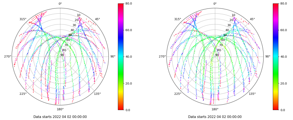
Skyplot for station SEV1. Parameter M1C Data file SEV100ESP_R_2022092.xtr Skyplot for station SEV1. Parameter M2C Data file SEV100ESP_R_2022092.xtr
