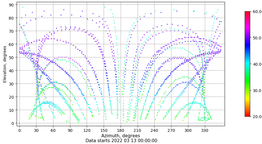
Azimuth-elevation plot for station SEV1. Signal to Noise S1C Data file SEV100ESP_R_2022072.xtr
