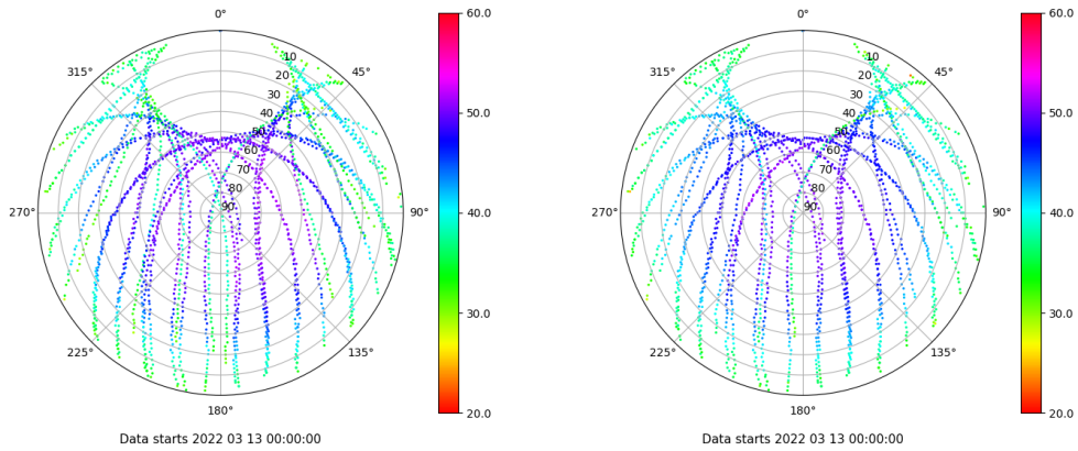
Skyplot for station SEV1. Signal to Noise S1C Data file SEV100ESP_R_2022072.xtr Skyplot for station SEV1. Signal to Noise S2C Data file SEV100ESP_R_2022072.xtr
