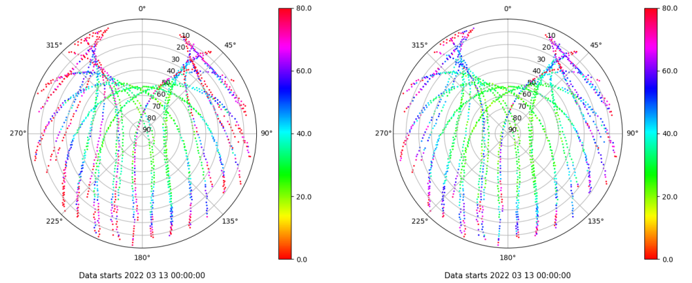
Skyplot for station SEV1. Parameter M1C Data file SEV100ESP_R_2022072.xtr Skyplot for station SEV1. Parameter M2C Data file SEV100ESP_R_2022072.xtr
