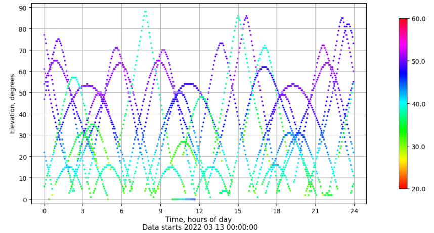
Time-elevation plot for station SEV1. Signal to Noise S1C Data file SEV100ESP_R_2022072.xtr
