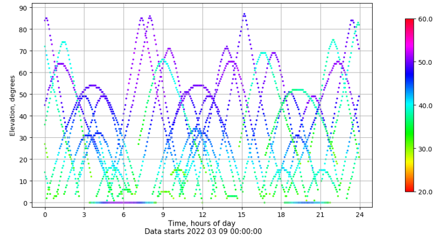
Time-elevation plot for station SEV1. Signal to Noise S1C Data file SEV100ESP_R_2022068.xtr
