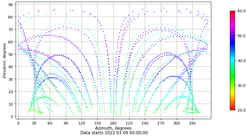
Azimuth-elevation plot for station SEV1. Signal to Noise S1C Data file SEV100ESP_R_2022068.xtr
