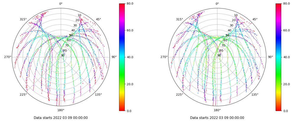
Skyplot for station SEV1. Parameter M1C Data file SEV100ESP_R_2022068.xtr Skyplot for station SEV1. Parameter M2C Data file SEV100ESP_R_2022068.xtr
