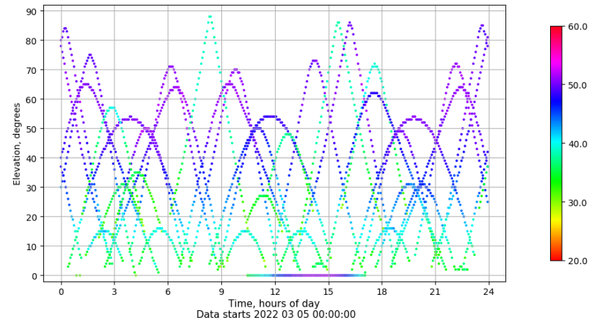
Time-elevation plot for station SEV1. Signal to Noise S1C Data file SEV100ESP_R_2022064.xtr
