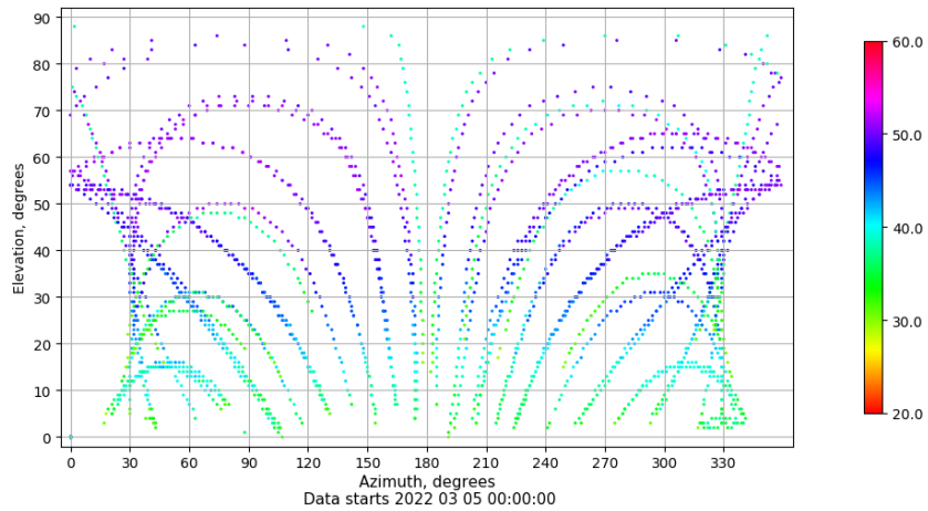
Azimuth-elevation plot for station SEV1. Signal to Noise S1C Data file SEV100ESP_R_2022064.xtr
