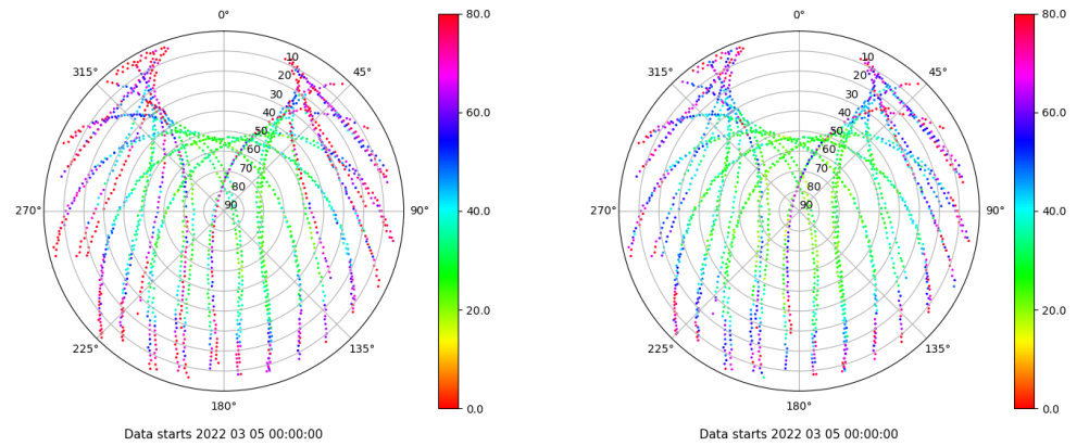
Skyplot for station SEV1. Parameter M1C Data file SEV100ESP_R_2022064.xtr Skyplot for station SEV1. Parameter M2C Data file SEV100ESP_R_2022064.xtr
