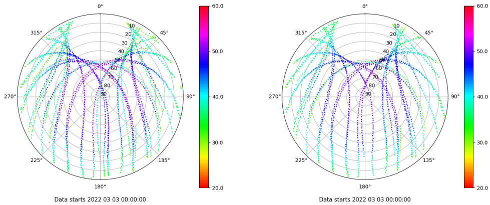
Skyplot for station SEV1. Signal to Noise S1C Data file SEV100ESP_R_2022062.xtr Skyplot for station SEV1. Signal to Noise S2C Data file SEV100ESP_R_2022062.xtr
