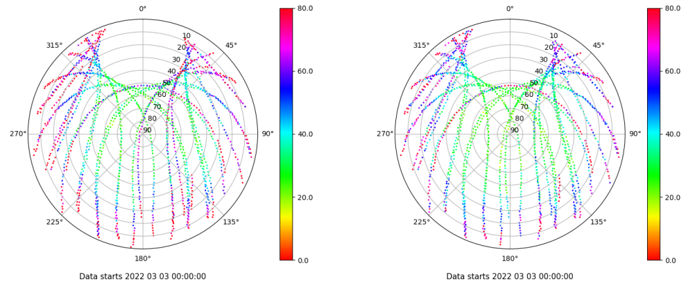
Skyplot for station SEV1. Parameter M1C Data file SEV100ESP_R_2022062.xtr Skyplot for station SEV1. Parameter M2C Data file SEV100ESP_R_2022062.xtr
