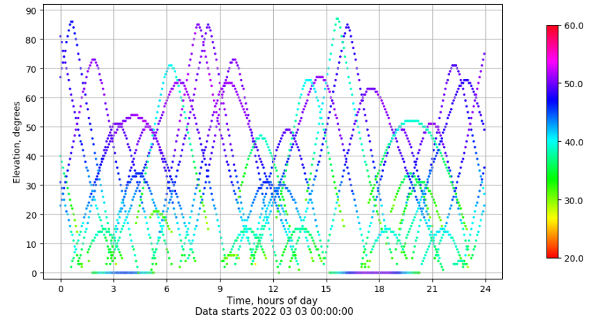
Time-elevation plot for station SEV1. Signal to Noise S1C Data file SEV100ESP_R_2022062.xtr
