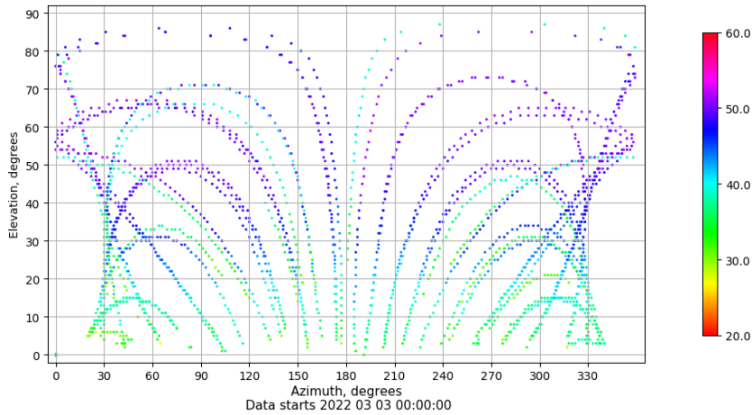
Azimuth-elevation plot for station SEV1. Signal to Noise S1C Data file SEV100ESP_R_2022062.xtr
