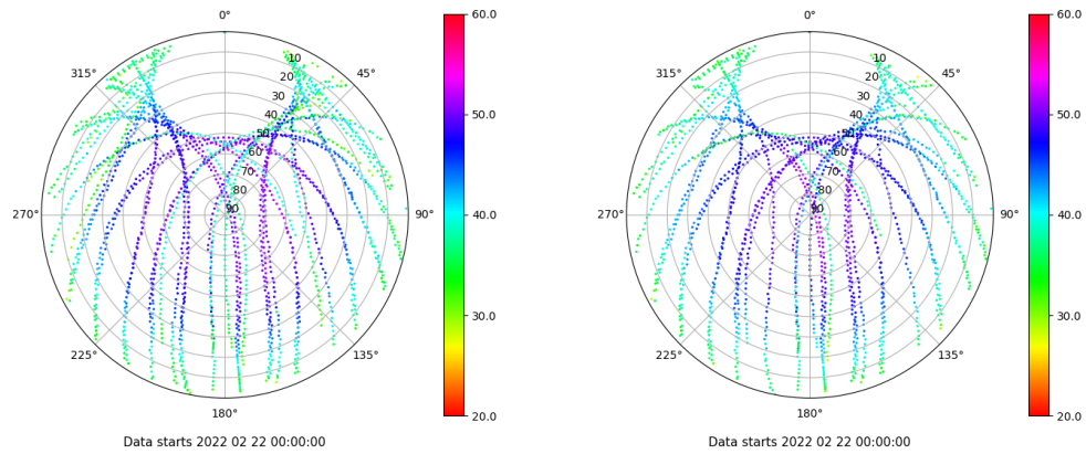
Skyplot for station SEV1. Signal to Noise S1C Data file SEV100ESP_R_2022053.xtr Skyplot for station SEV1. Signal to Noise S2C Data file SEV100ESP_R_2022053.xtr
