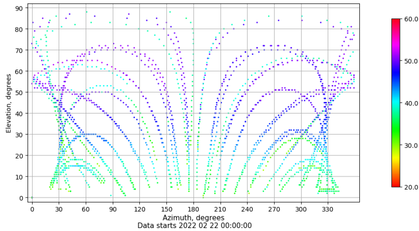
Azimuth-elevation plot for station SEV1. Signal to Noise S1C Data file SEV100ESP_R_2022053.xtr
