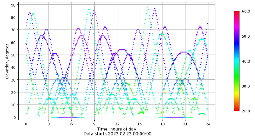
Time-elevation plot for station SEV1. Signal to Noise S1C Data file SEV100ESP_R_2022053.xtr
