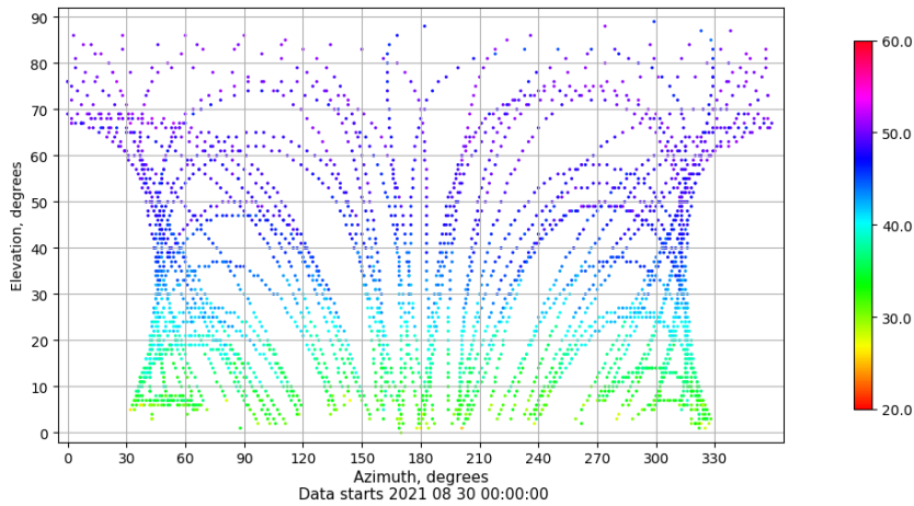
Azimuth-elevation plot for station SEV1. Signal to Noise S1C Data file SEV100ESP_R_2021242.xtr
