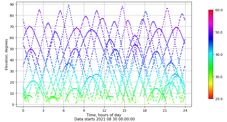
Time-elevation plot for station SEV1. Signal to Noise S1C Data file SEV100ESP_R_2021242.xtr
