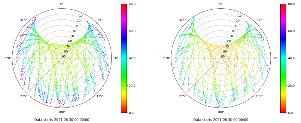
Skyplot for station SEV1. Parameter M1C Data file SEV100ESP_R_2021242.xtr Skyplot for station SEV1. Parameter M2X Data file SEV100ESP_R_2021242.xtr
