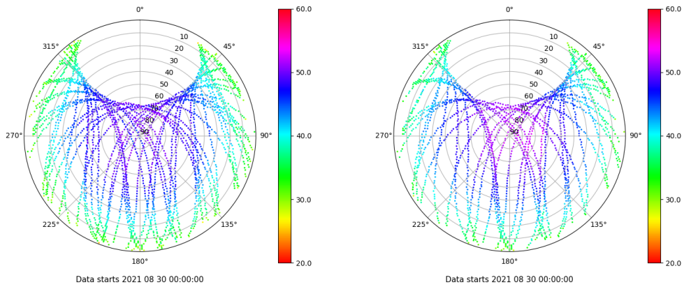
Skyplot for station SEV1. Signal to Noise S1C Data file SEV100ESP_R_2021242.xtr Skyplot for station SEV1. Signal to Noise S2X Data file SEV100ESP_R_2021242.xtr
