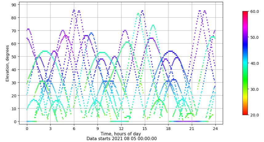
Time-elevation plot for station SEV1. Signal to Noise S1C Data file SEV100ESP_R_2021217.xtr
