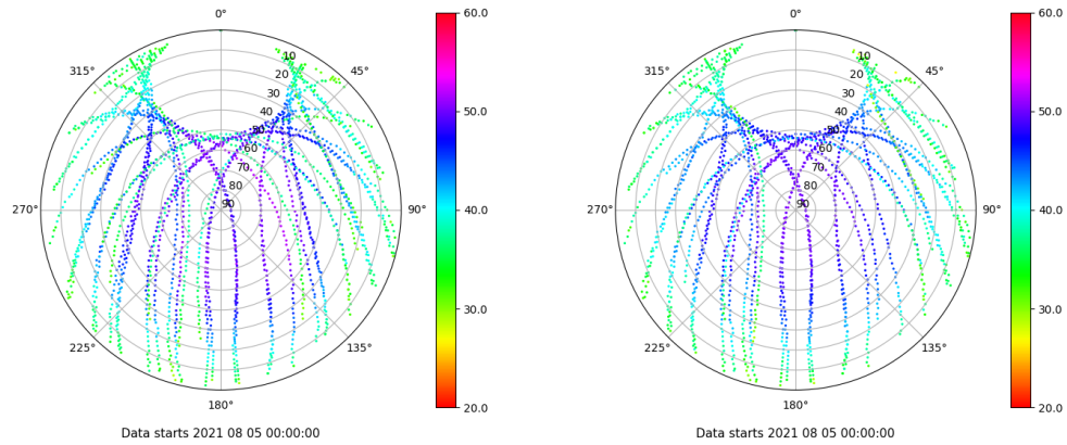
Skyplot for station SEV1. Signal to Noise S1C Data file SEV100ESP_R_2021217.xtr Skyplot for station SEV1. Signal to Noise S2C Data file SEV100ESP_R_2021217.xtr
