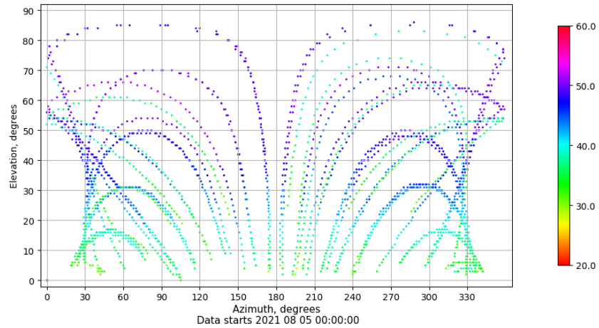
Azimuth-elevation plot for station SEV1. Signal to Noise S1C Data file SEV100ESP_R_2021217.xtr
