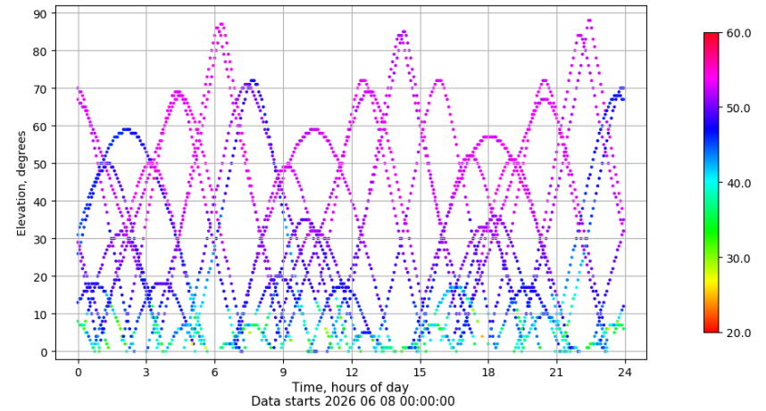
Time-elevation plot for station SALA. Signal to Noise S1C Data file SALA00ESP_R_2026159.xtr
