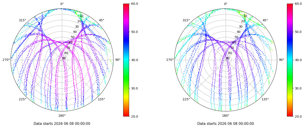
Skyplot for station SALA. Signal to Noise S1C Data file SALA00ESP_R_2026159.xtr Skyplot for station SALA. Signal to Noise S2P Data file SALA00ESP_R_2026159.xtr
