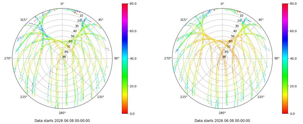
Skyplot for station SALA. Parameter M1C Data file SALA00ESP_R_2026159.xtr Skyplot for station SALA. Parameter M2P Data file SALA00ESP_R_2026159.xtr
