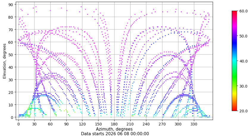
Azimuth-elevation plot for station SALA. Signal to Noise S1C Data file SALA00ESP_R_2026159.xtr
