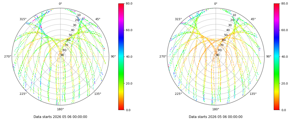
Skyplot for station SALA. Parameter M1C Data file SALA00ESP_R_2026126.xtr Skyplot for station SALA. Parameter M2P Data file SALA00ESP_R_2026126.xtr
