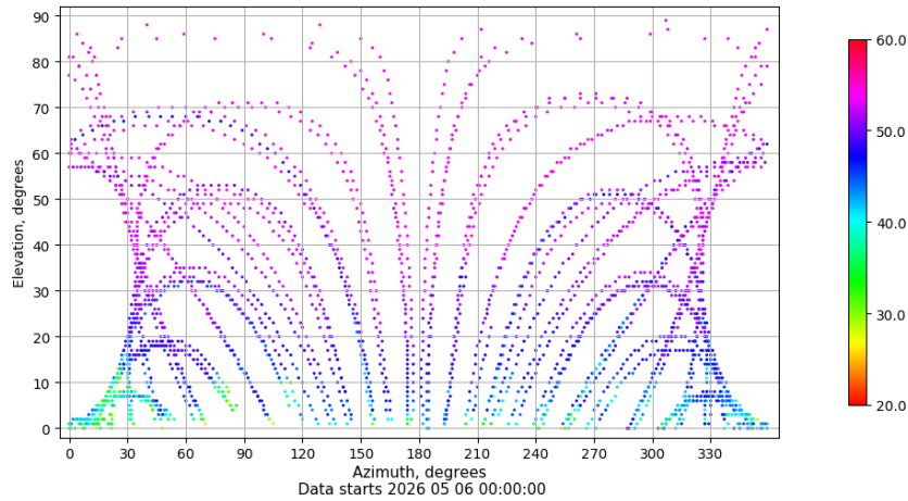
Azimuth-elevation plot for station SALA. Signal to Noise S1C Data file SALA00ESP_R_2026126.xtr
