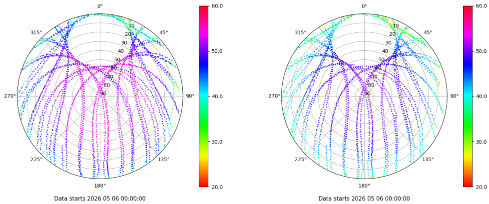
Skyplot for station SALA. Signal to Noise S1C Data file SALA00ESP_R_2026126.xtr Skyplot for station SALA. Signal to Noise S2P Data file SALA00ESP_R_2026126.xtr
