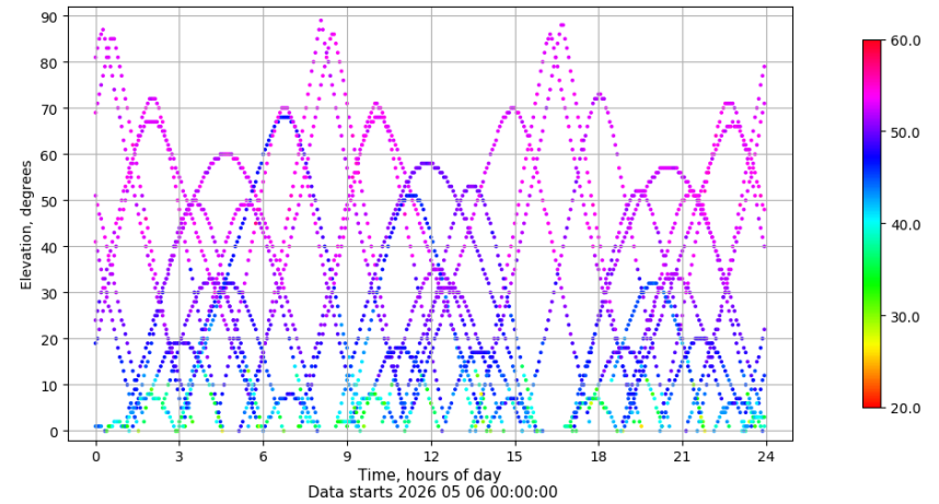
Time-elevation plot for station SALA. Signal to Noise S1C Data file SALA00ESP_R_2026126.xtr
