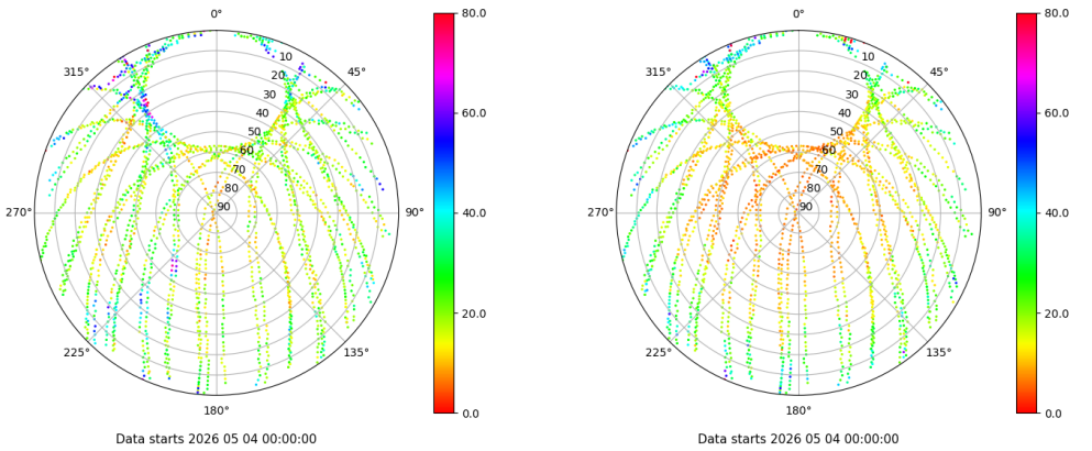
Skyplot for station SALA. Parameter M1C Data file SALA00ESP_R_2026124.xtr Skyplot for station SALA. Parameter M2P Data file SALA00ESP_R_2026124.xtr
