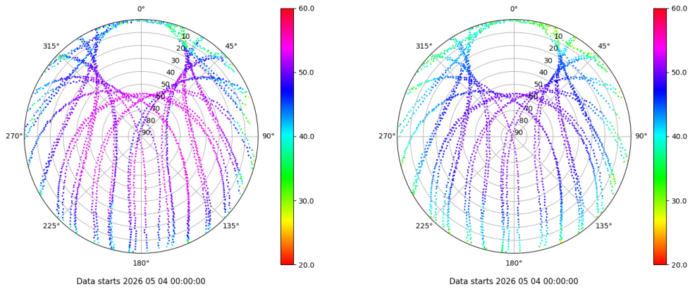
Skyplot for station SALA. Signal to Noise S1C Data file SALA00ESP_R_2026124.xtr Skyplot for station SALA. Signal to Noise S2P Data file SALA00ESP_R_2026124.xtr
