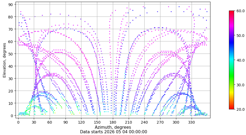
Azimuth-elevation plot for station SALA. Signal to Noise S1C Data file SALA00ESP_R_2026124.xtr
