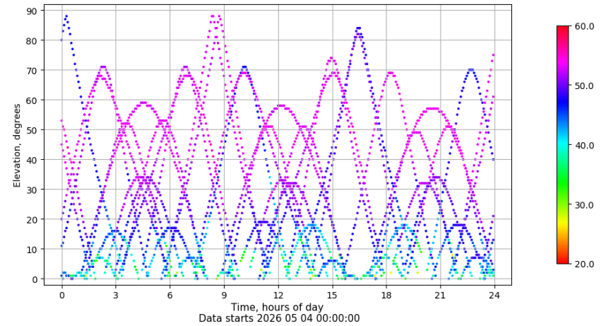
Time-elevation plot for station SALA. Signal to Noise S1C Data file SALA00ESP_R_2026124.xtr
