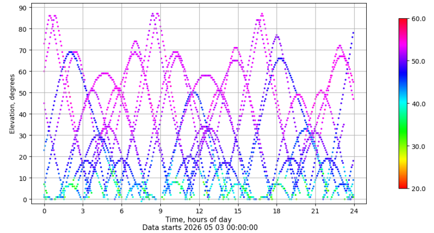
Time-elevation plot for station SALA. Signal to Noise S1C Data file SALA00ESP_R_2026123.xtr
