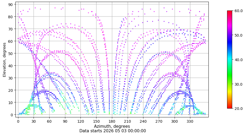
Azimuth-elevation plot for station SALA. Signal to Noise S1C Data file SALA00ESP_R_2026123.xtr
