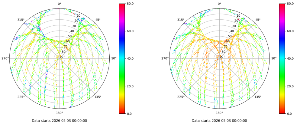
Skyplot for station SALA. Parameter M1C Data file SALA00ESP_R_2026123.xtr Skyplot for station SALA. Parameter M2P Data file SALA00ESP_R_2026123.xtr
