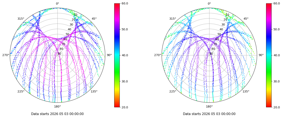
Skyplot for station SALA. Signal to Noise S1C Data file SALA00ESP_R_2026123.xtr Skyplot for station SALA. Signal to Noise S2P Data file SALA00ESP_R_2026123.xtr
