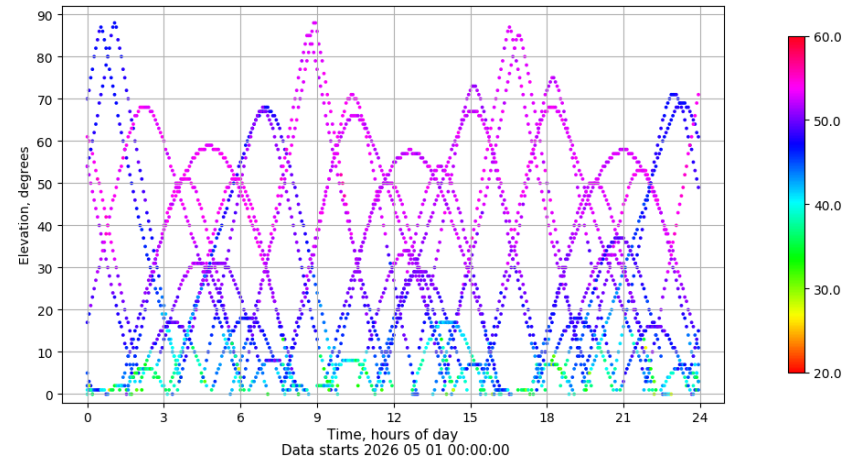
Time-elevation plot for station SALA. Signal to Noise S1C Data file SALA00ESP_R_2026121.xtr
