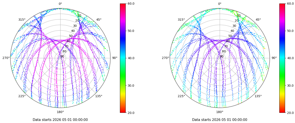
Skyplot for station SALA. Signal to Noise S1C Data file SALA00ESP_R_2026121.xtr Skyplot for station SALA. Signal to Noise S2P Data file SALA00ESP_R_2026121.xtr
