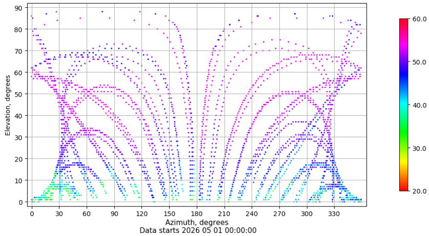
Azimuth-elevation plot for station SALA. Signal to Noise S1C Data file SALA00ESP_R_2026121.xtr
