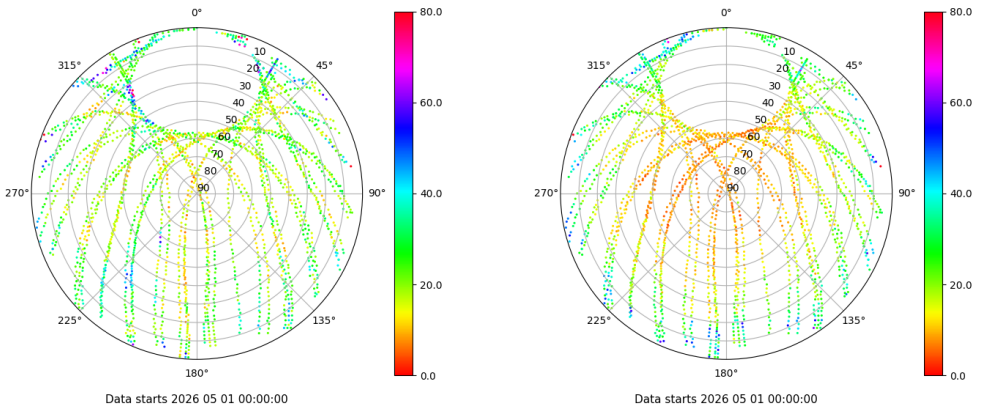
Skyplot for station SALA. Parameter M1C Data file SALA00ESP_R_2026121.xtr Skyplot for station SALA. Parameter M2P Data file SALA00ESP_R_2026121.xtr
