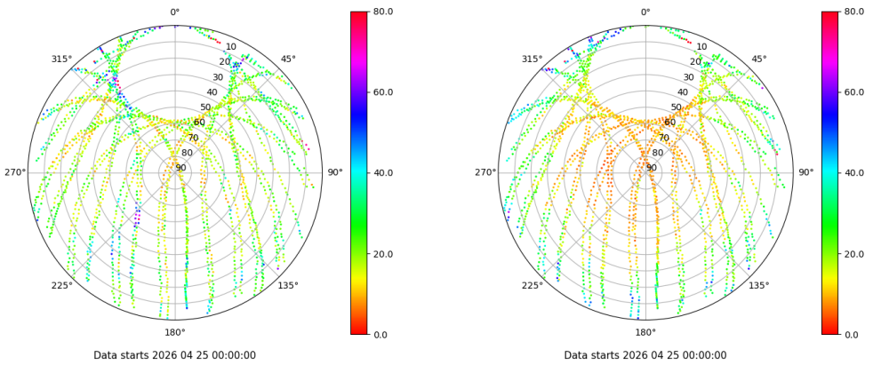
Skyplot for station SALA. Parameter M1C Data file SALA00ESP_R_2026115.xtr Skyplot for station SALA. Parameter M2P Data file SALA00ESP_R_2026115.xtr
