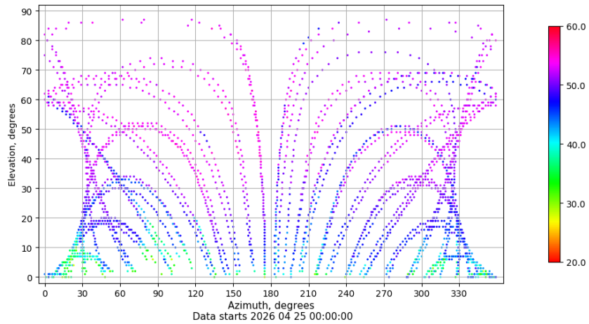
Azimuth-elevation plot for station SALA. Signal to Noise S1C Data file SALA00ESP_R_2026115.xtr
