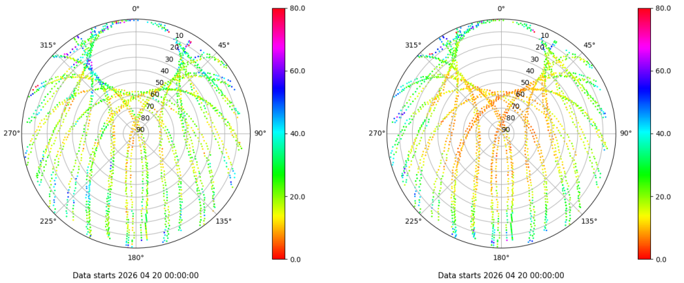
Skyplot for station SALA. Parameter M1C Data file SALA00ESP_R_2026110.xtr Skyplot for station SALA. Parameter M2P Data file SALA00ESP_R_2026110.xtr
