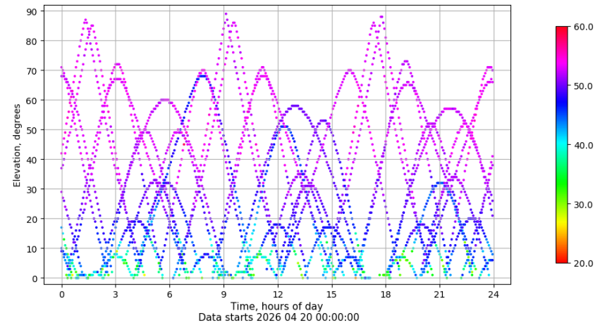
Time-elevation plot for station SALA. Signal to Noise S1C Data file SALA00ESP_R_2026110.xtr
