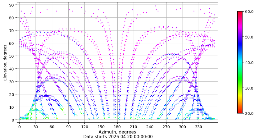
Azimuth-elevation plot for station SALA. Signal to Noise S1C Data file SALA00ESP_R_2026110.xtr
