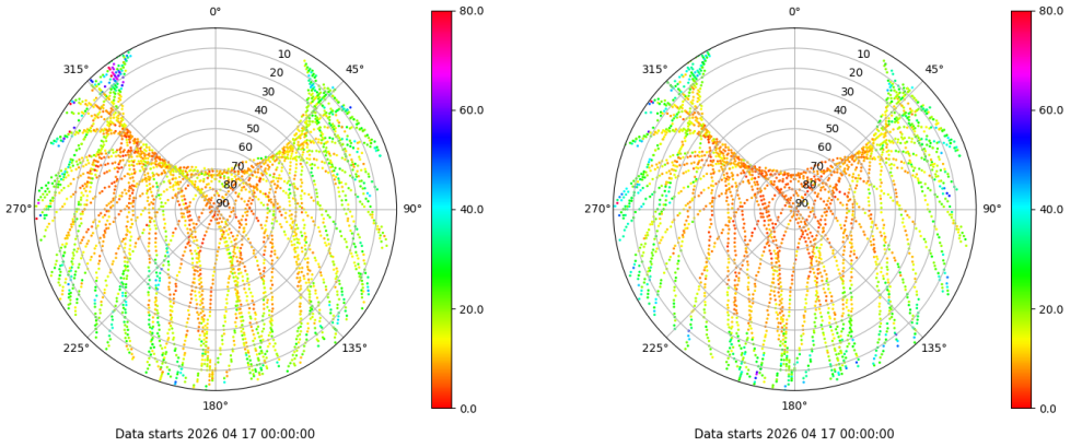
Skyplot for station SALA. Parameter M1C Data file SALA00ESP_R_2026107.xtr Skyplot for station SALA. Parameter M2S Data file SALA00ESP_R_2026107.xtr
