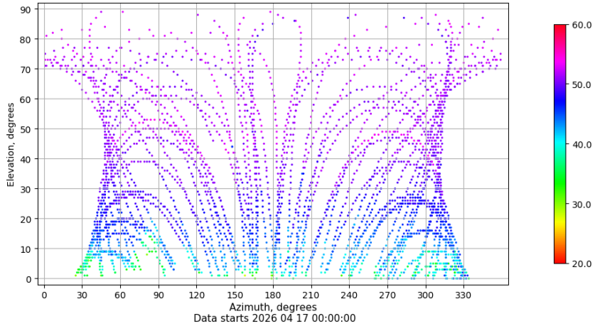
Azimuth-elevation plot for station SALA. Signal to Noise S1C Data file SALA00ESP_R_2026107.xtr
