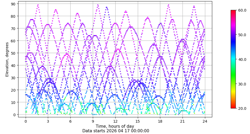
Time-elevation plot for station SALA. Signal to Noise S1C Data file SALA00ESP_R_2026107.xtr
