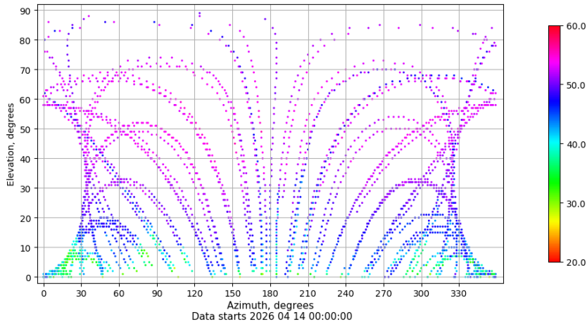
Azimuth-elevation plot for station SALA. Signal to Noise S1C Data file SALA00ESP_R_2026104.xtr
