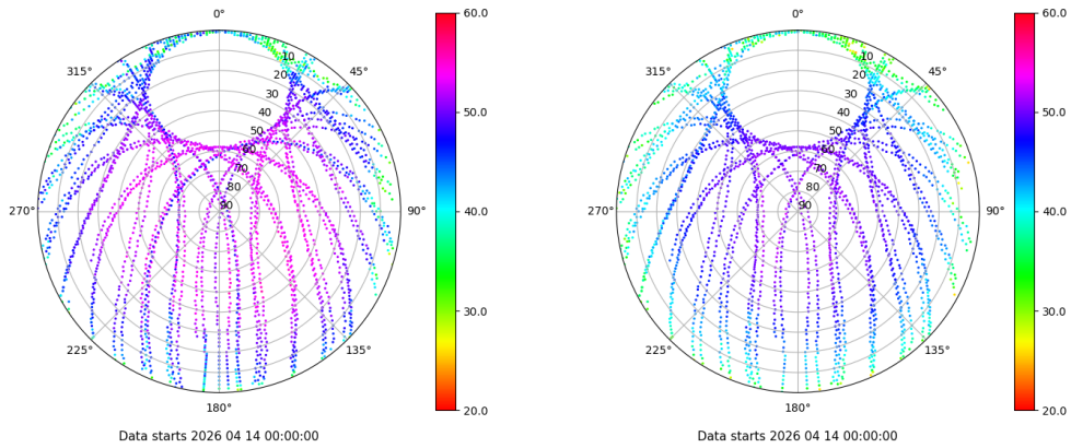
Skyplot for station SALA. Signal to Noise S1C Data file SALA00ESP_R_2026104.xtr Skyplot for station SALA. Signal to Noise S2P Data file SALA00ESP_R_2026104.xtr
