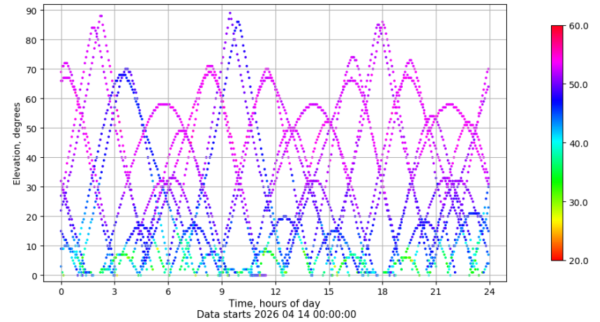
Time-elevation plot for station SALA. Signal to Noise S1C Data file SALA00ESP_R_2026104.xtr
