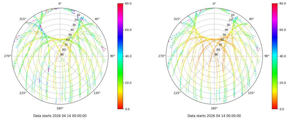
Skyplot for station SALA. Parameter M1C Data file SALA00ESP_R_2026104.xtr Skyplot for station SALA. Parameter M2P Data file SALA00ESP_R_2026104.xtr
