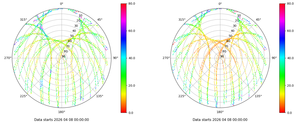
Skyplot for station SALA. Parameter M1C Data file SALA00ESP_R_2026098.xtr Skyplot for station SALA. Parameter M2P Data file SALA00ESP_R_2026098.xtr
