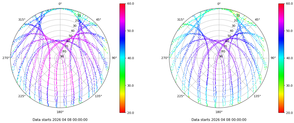
Skyplot for station SALA. Signal to Noise S1C Data file SALA00ESP_R_2026098.xtr Skyplot for station SALA. Signal to Noise S2P Data file SALA00ESP_R_2026098.xtr
