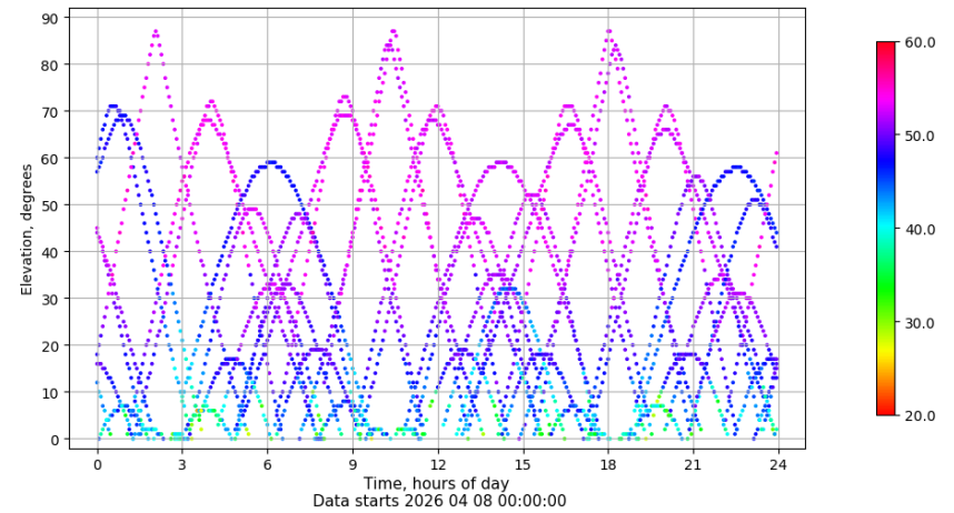
Time-elevation plot for station SALA. Signal to Noise S1C Data file SALA00ESP_R_2026098.xtr
