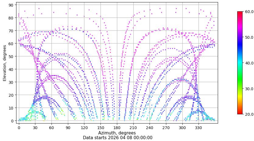
Azimuth-elevation plot for station SALA. Signal to Noise S1C Data file SALA00ESP_R_2026098.xtr
