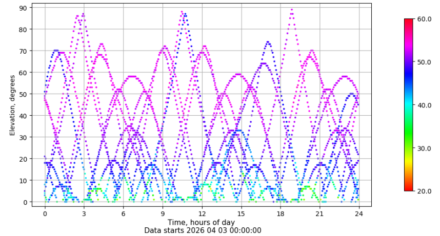
Time-elevation plot for station SALA. Signal to Noise S1C Data file SALA00ESP_R_2026093.xtr
