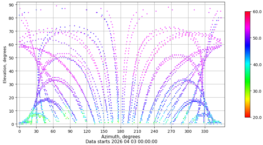
Azimuth-elevation plot for station SALA. Signal to Noise S1C Data file SALA00ESP_R_2026093.xtr
