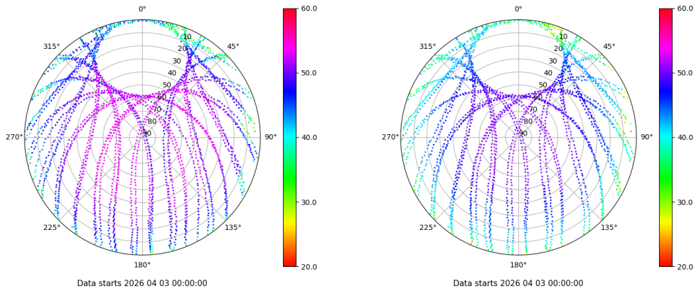
Skyplot for station SALA. Signal to Noise S1C Data file SALA00ESP_R_2026093.xtr Skyplot for station SALA. Signal to Noise S2P Data file SALA00ESP_R_2026093.xtr
