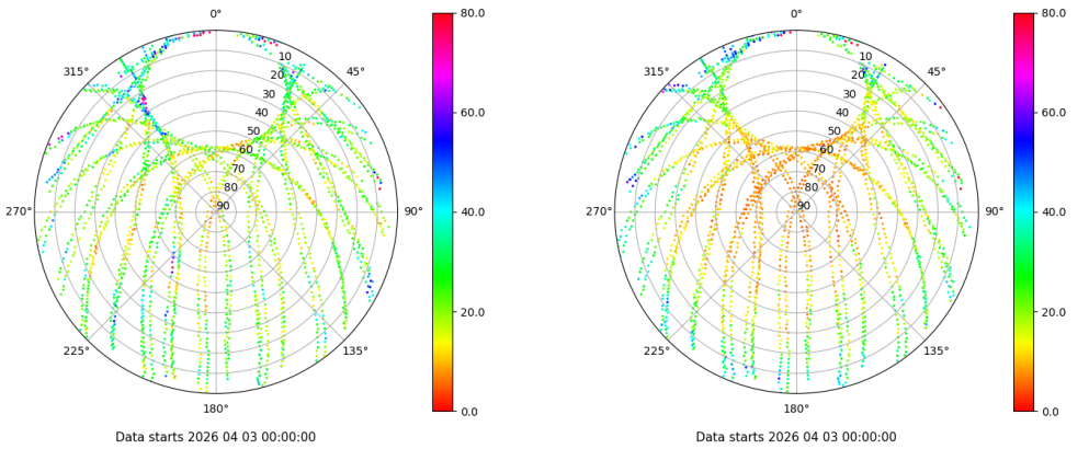
Skyplot for station SALA. Parameter M1C Data file SALA00ESP_R_2026093.xtr Skyplot for station SALA. Parameter M2P Data file SALA00ESP_R_2026093.xtr
