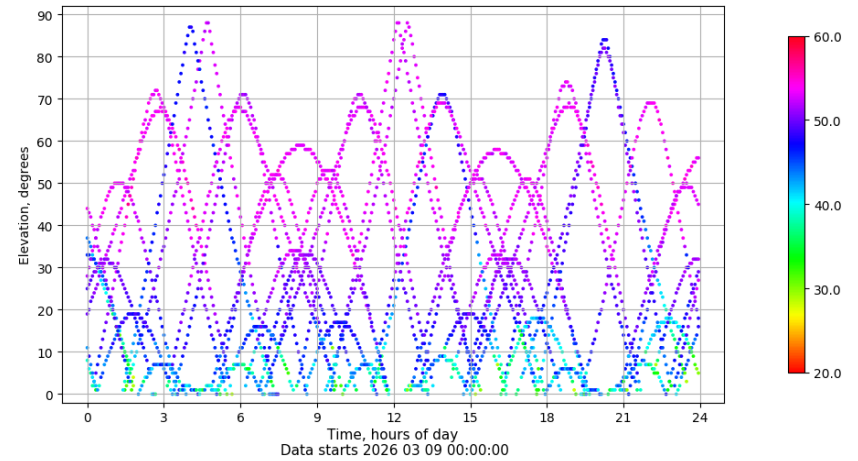
Time-elevation plot for station SALA. Signal to Noise S1C Data file SALA00ESP_R_2026068.xtr
