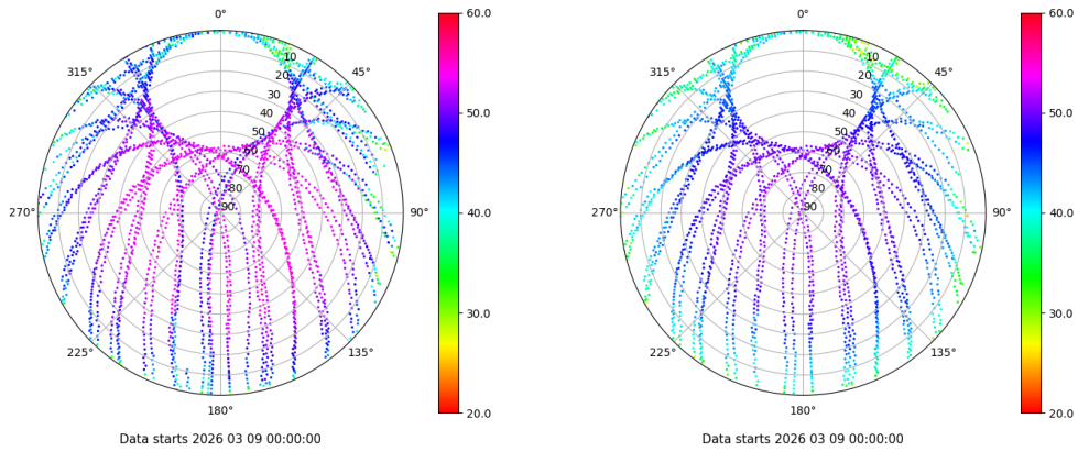
Skyplot for station SALA. Signal to Noise S1C Data file SALA00ESP_R_2026068.xtr Skyplot for station SALA. Signal to Noise S2P Data file SALA00ESP_R_2026068.xtr
