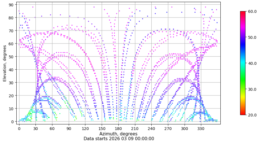
Azimuth-elevation plot for station SALA. Signal to Noise S1C Data file SALA00ESP_R_2026068.xtr
