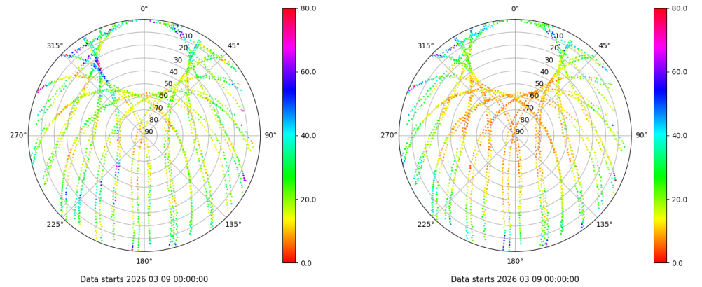
Skyplot for station SALA. Parameter M1C Data file SALA00ESP_R_2026068.xtr Skyplot for station SALA. Parameter M2P Data file SALA00ESP_R_2026068.xtr
