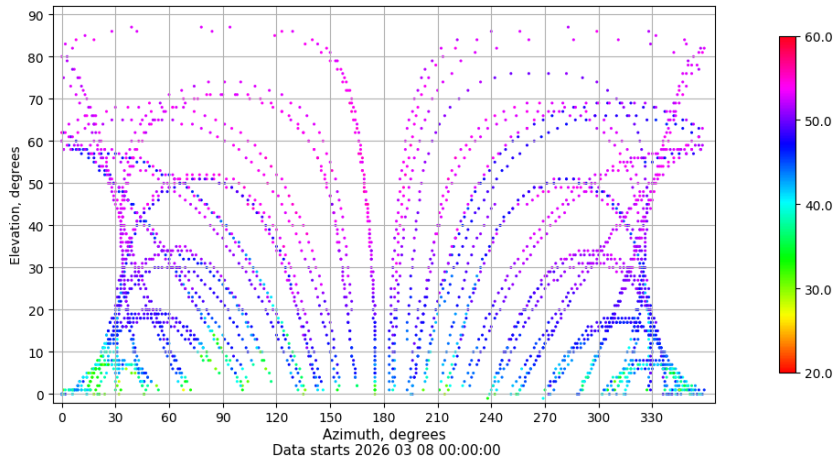
Azimuth-elevation plot for station SALA. Signal to Noise S1C Data file SALA00ESP_R_2026067.xtr
