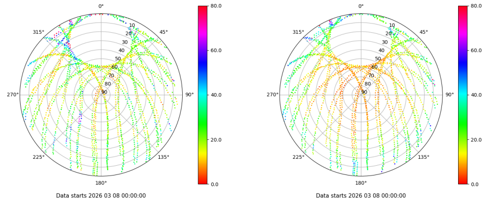
Skyplot for station SALA. Parameter M1C Data file SALA00ESP_R_2026067.xtr Skyplot for station SALA. Parameter M2P Data file SALA00ESP_R_2026067.xtr
