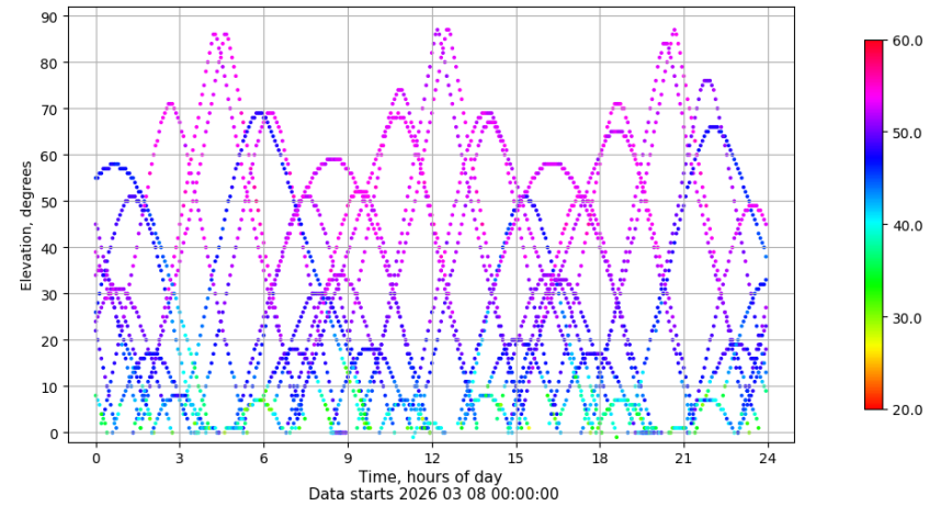
Time-elevation plot for station SALA. Signal to Noise S1C Data file SALA00ESP_R_2026067.xtr
