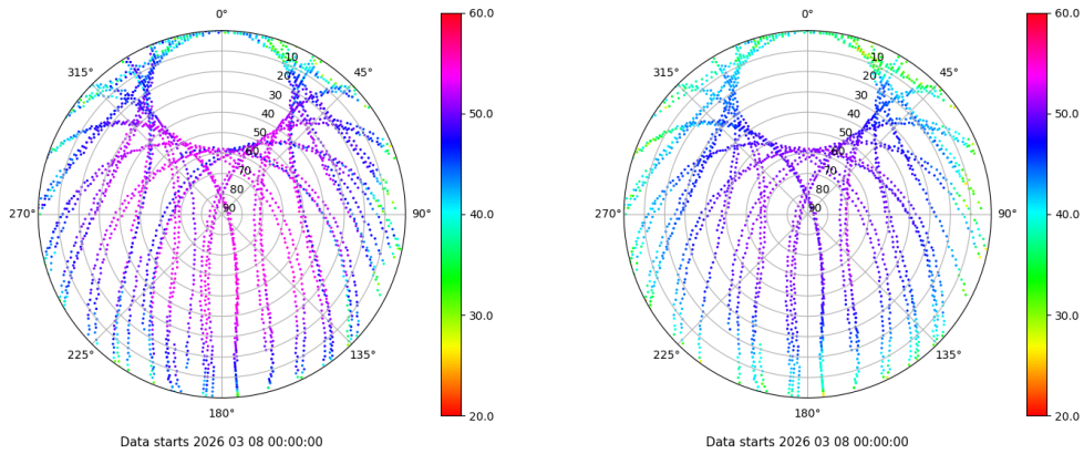
Skyplot for station SALA. Signal to Noise S1C Data file SALA00ESP_R_2026067.xtr Skyplot for station SALA. Signal to Noise S2P Data file SALA00ESP_R_2026067.xtr
