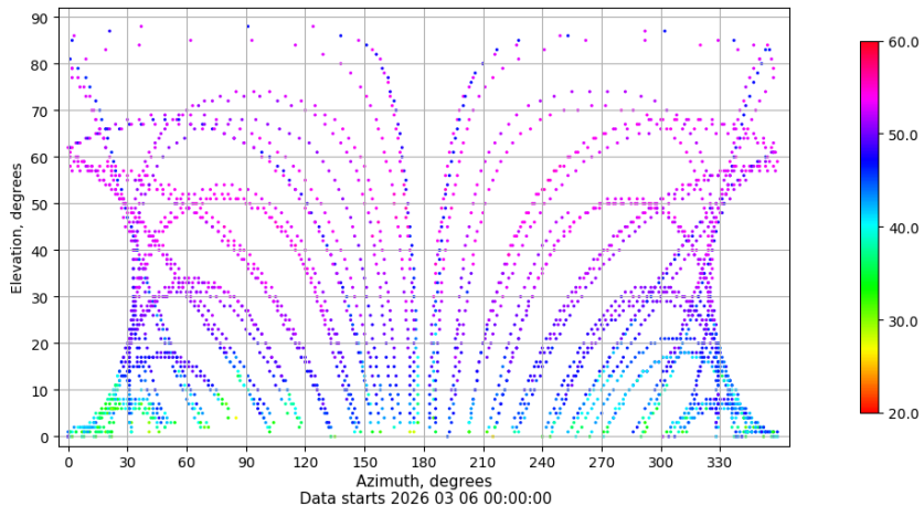
Azimuth-elevation plot for station SALA. Signal to Noise S1C Data file SALA00ESP_R_2026065.xtr
