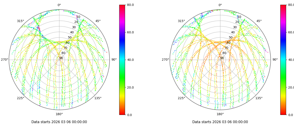
Skyplot for station SALA. Parameter M1C Data file SALA00ESP_R_2026065.xtr Skyplot for station SALA. Parameter M2P Data file SALA00ESP_R_2026065.xtr
