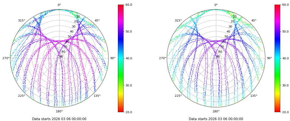
Skyplot for station SALA. Signal to Noise S1C Data file SALA00ESP_R_2026065.xtr Skyplot for station SALA. Signal to Noise S2P Data file SALA00ESP_R_2026065.xtr
