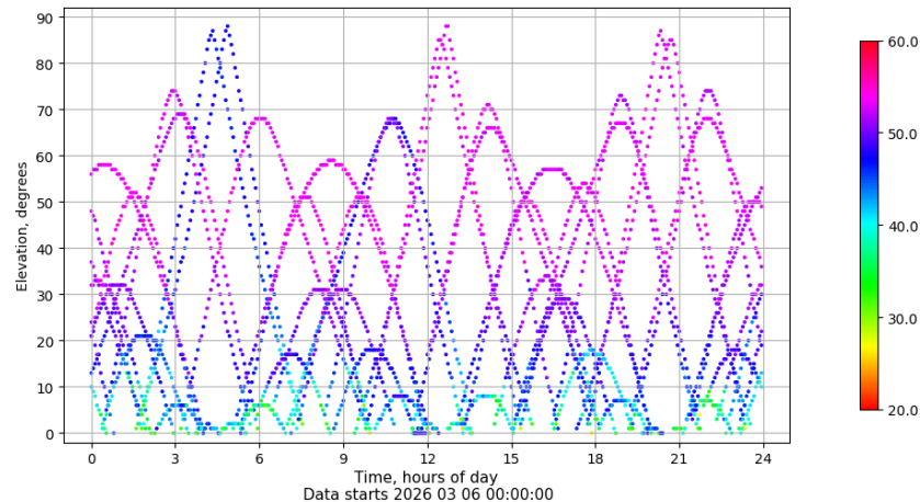
Time-elevation plot for station SALA. Signal to Noise S1C Data file SALA00ESP_R_2026065.xtr
