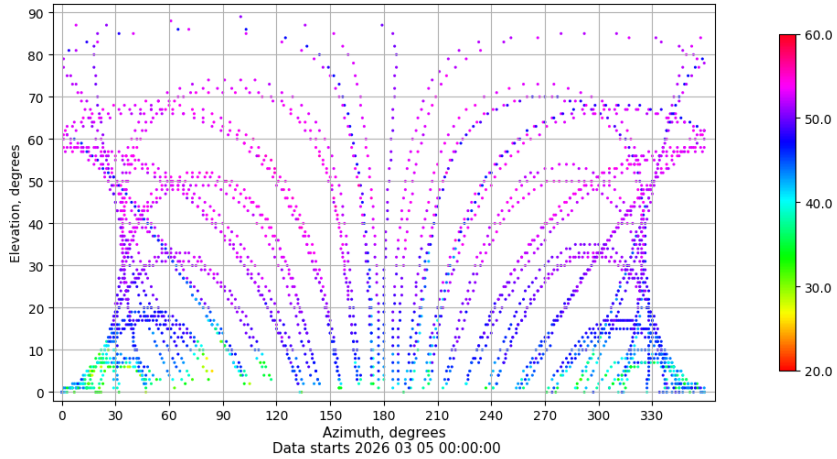
Azimuth-elevation plot for station SALA. Signal to Noise S1C Data file SALA00ESP_R_2026064.xtr
