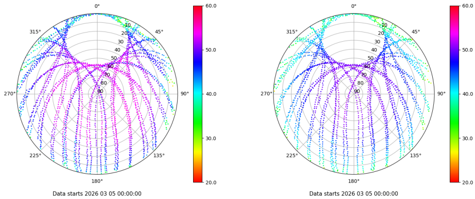
Skyplot for station SALA. Signal to Noise S1C Data file SALA00ESP_R_2026064.xtr Skyplot for station SALA. Signal to Noise S2P Data file SALA00ESP_R_2026064.xtr
