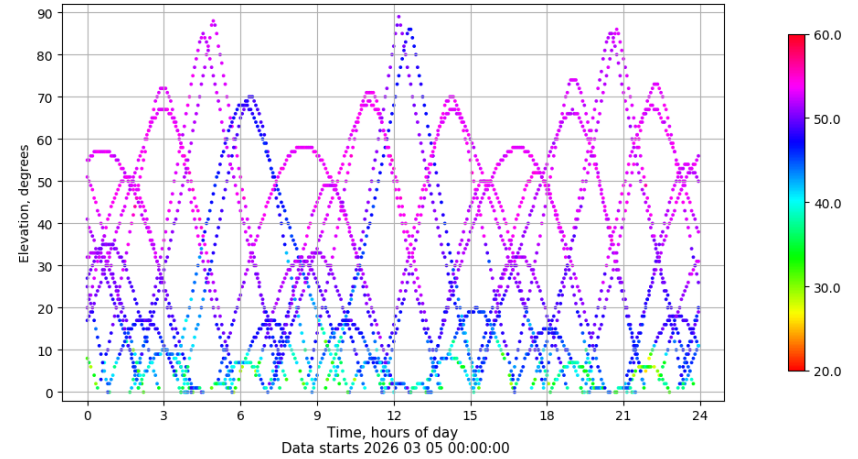
Time-elevation plot for station SALA. Signal to Noise S1C Data file SALA00ESP_R_2026064.xtr
