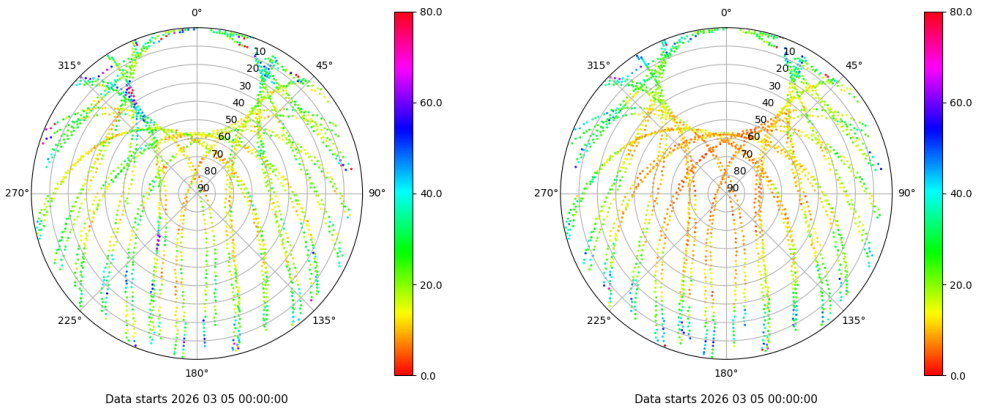
Skyplot for station SALA. Parameter M1C Data file SALA00ESP_R_2026064.xtr Skyplot for station SALA. Parameter M2P Data file SALA00ESP_R_2026064.xtr
