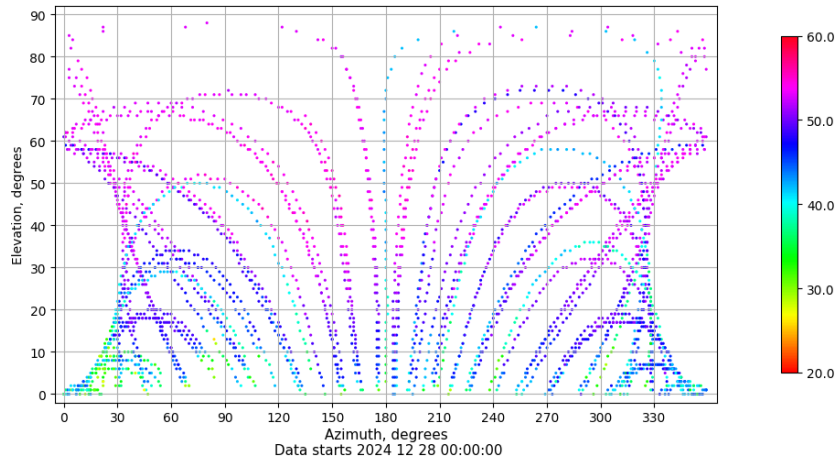
Azimuth-elevation plot for station SALA. Signal to Noise S1C Data file SALA00ESP_R_2024363.xtr
