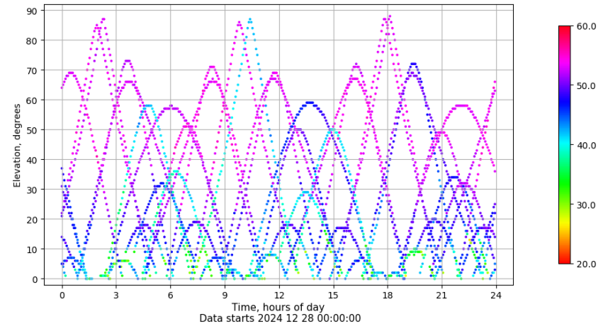
Time-elevation plot for station SALA. Signal to Noise S1C Data file SALA00ESP_R_2024363.xtr
