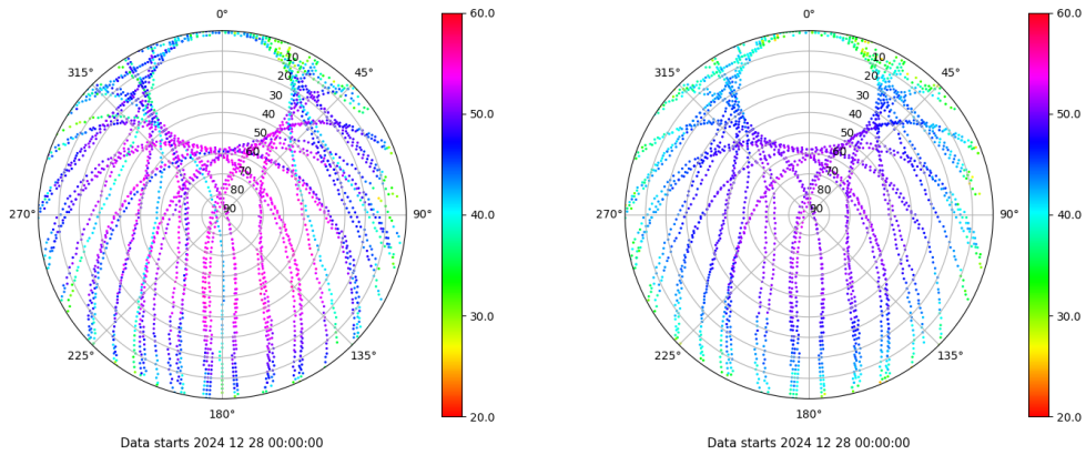
Skyplot for station SALA. Signal to Noise S1C Data file SALA00ESP_R_2024363.xtr Skyplot for station SALA. Signal to Noise S2P Data file SALA00ESP_R_2024363.xtr
