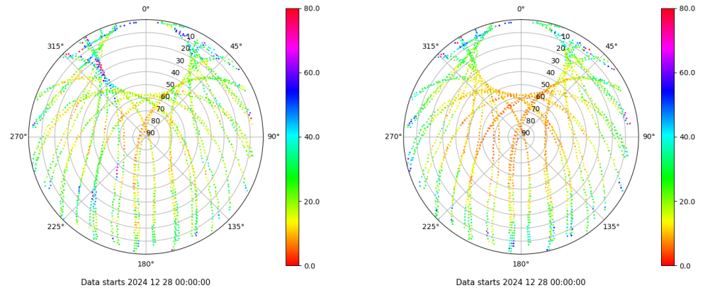
Skyplot for station SALA. Parameter M1C Data file SALA00ESP_R_2024363.xtr Skyplot for station SALA. Parameter M2P Data file SALA00ESP_R_2024363.xtr
