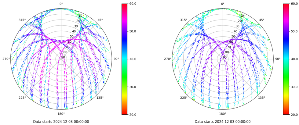
Skyplot for station SALA. Signal to Noise S1C Data file SALA00ESP_R_2024338.xtr Skyplot for station SALA. Signal to Noise S2P Data file SALA00ESP_R_2024338.xtr
