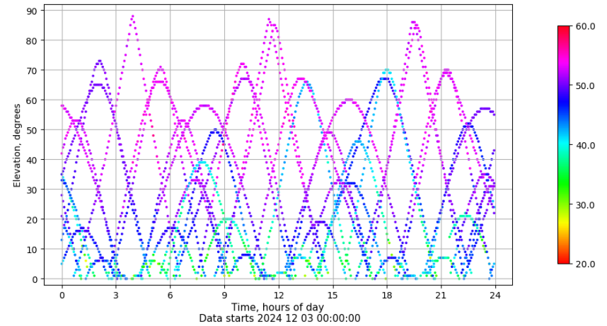
Time-elevation plot for station SALA. Signal to Noise S1C Data file SALA00ESP_R_2024338.xtr
