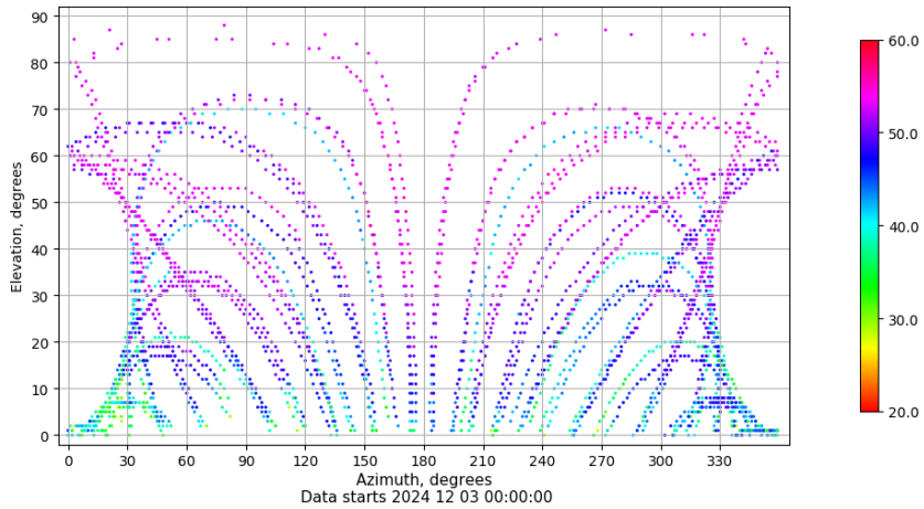
Azimuth-elevation plot for station SALA. Signal to Noise S1C Data file SALA00ESP_R_2024338.xtr
