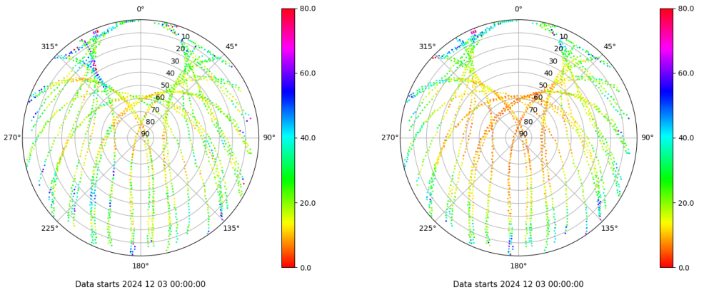
Skyplot for station SALA. Parameter M1C Data file SALA00ESP_R_2024338.xtr Skyplot for station SALA. Parameter M2P Data file SALA00ESP_R_2024338.xtr
