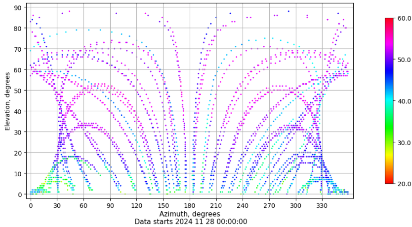
Azimuth-elevation plot for station SALA. Signal to Noise S1C Data file SALA00ESP_R_2024333.xtr
