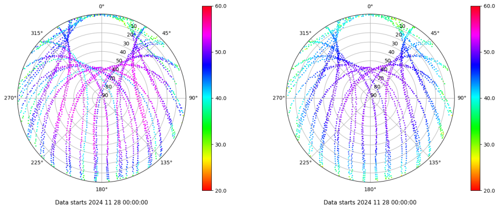
Skyplot for station SALA. Signal to Noise S1C Data file SALA00ESP_R_2024333.xtr Skyplot for station SALA. Signal to Noise S2P Data file SALA00ESP_R_2024333.xtr
