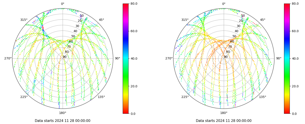
Skyplot for station SALA. Parameter M1C Data file SALA00ESP_R_2024333.xtr Skyplot for station SALA. Parameter M2P Data file SALA00ESP_R_2024333.xtr
