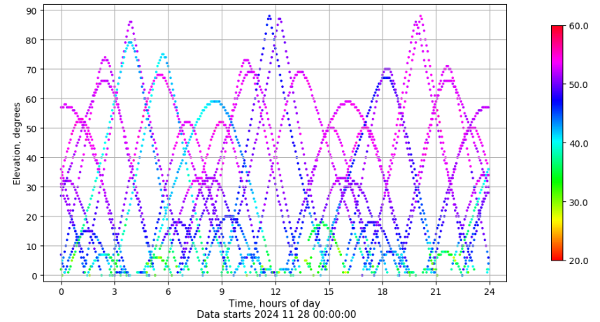
Time-elevation plot for station SALA. Signal to Noise S1C Data file SALA00ESP_R_2024333.xtr
