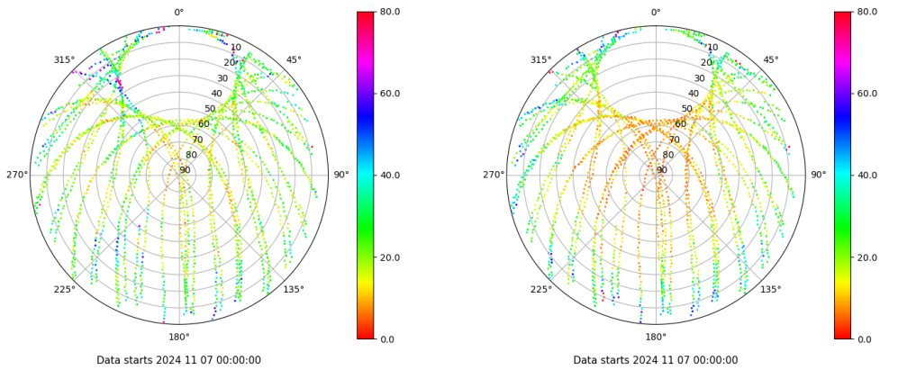
Skyplot for station SALA. Parameter M1C Data file SALA00ESP_R_2024312.xtr Skyplot for station SALA. Parameter M2P Data file SALA00ESP_R_2024312.xtr
