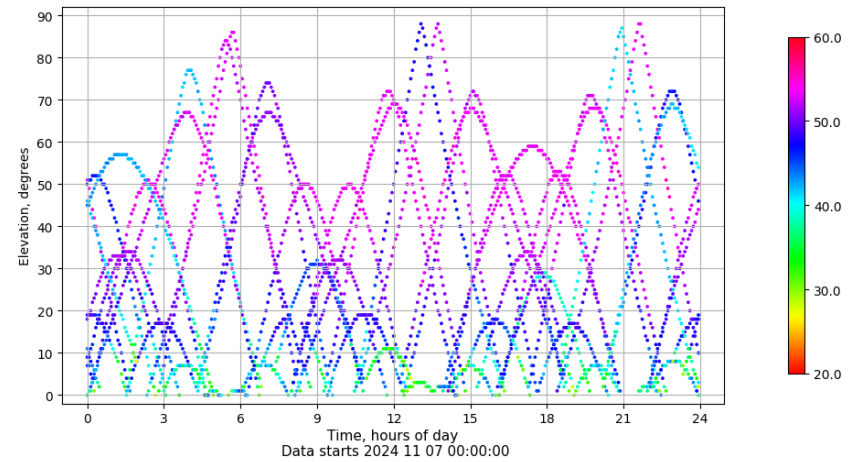
Time-elevation plot for station SALA. Signal to Noise S1C Data file SALA00ESP_R_2024312.xtr
