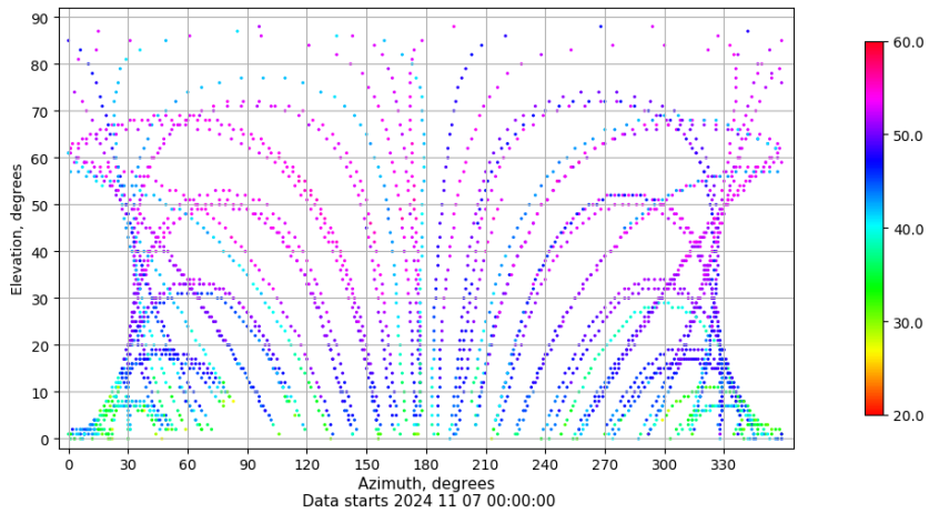
Azimuth-elevation plot for station SALA. Signal to Noise S1C Data file SALA00ESP_R_2024312.xtr
