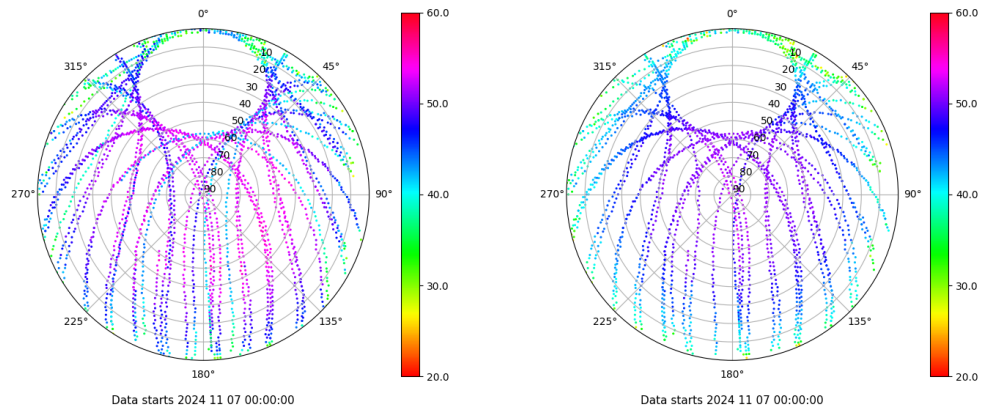
Skyplot for station SALA. Signal to Noise S1C Data file SALA00ESP_R_2024312.xtr Skyplot for station SALA. Signal to Noise S2P Data file SALA00ESP_R_2024312.xtr
