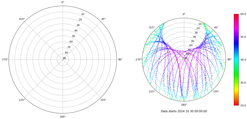
Skyplot for station SALA. Signal to Noise S1C Data file SALA00ESP_R_2024304.xtr Skyplot for station SALA. Signal to Noise S2S Data file SALA00ESP_R_2024304.xtr
