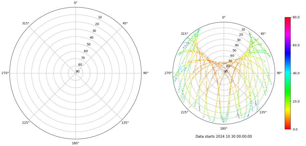
Skyplot for station SALA. Parameter M1C Data file SALA00ESP_R_2024304.xtr Skyplot for station SALA. Parameter M2S Data file SALA00ESP_R_2024304.xtr
