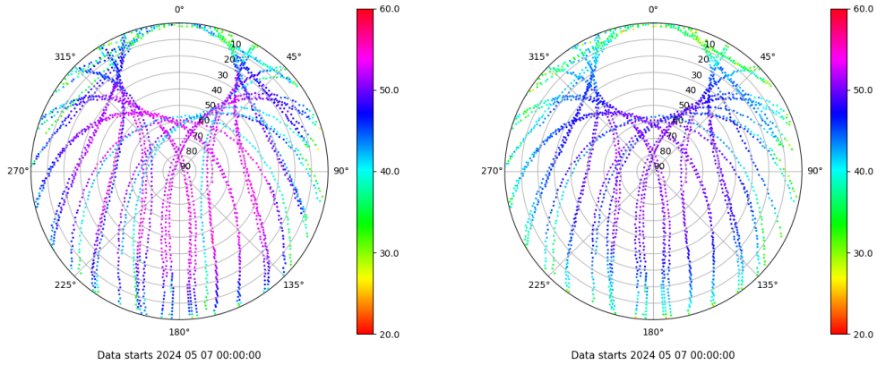
Skyplot for station SALA. Signal to Noise S1C Data file SALA00ESP_R_2024128.xtr Skyplot for station SALA. Signal to Noise S2P Data file SALA00ESP_R_2024128.xtr
