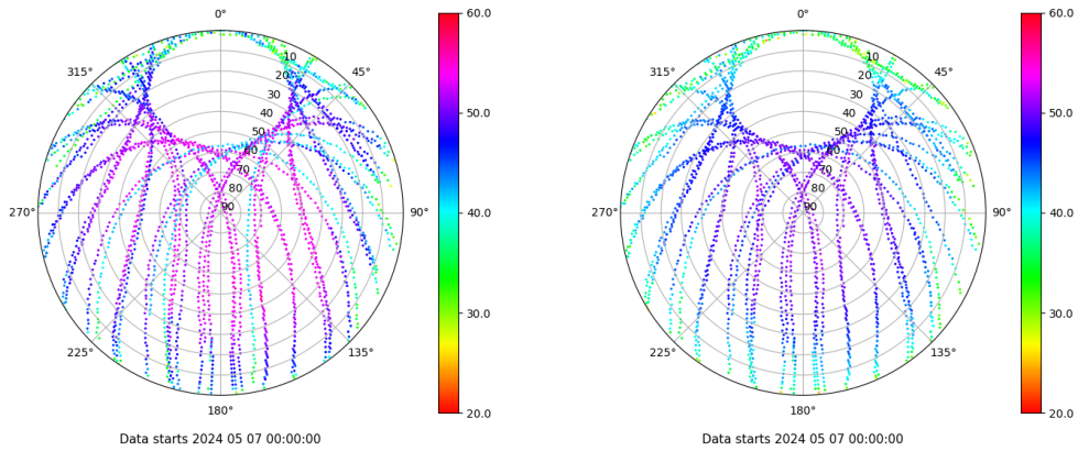
Skyplot for station SALA. Signal to Noise S1C Data file SALA00ESP_R_2024128.xtr Skyplot for station SALA. Signal to Noise S2P Data file SALA00ESP_R_2024128.xtr
