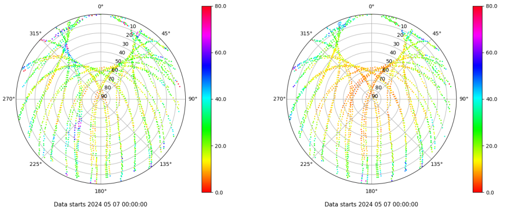
Skyplot for station SALA. Parameter M1C Data file SALA00ESP_R_2024128.xtr Skyplot for station SALA. Parameter M2P Data file SALA00ESP_R_2024128.xtr
