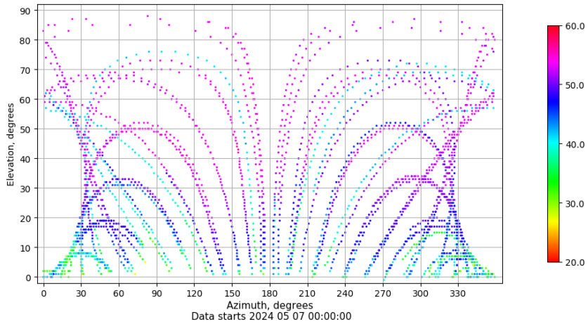
Azimuth-elevation plot for station SALA. Signal to Noise S1C Data file SALA00ESP_R_2024128.xtr
