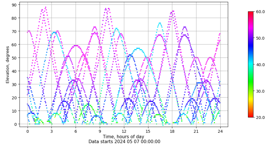
Time-elevation plot for station SALA. Signal to Noise S1C Data file SALA00ESP_R_2024128.xtr
