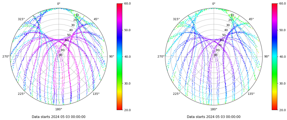
Skyplot for station SALA. Signal to Noise S1C Data file SALA00ESP_R_2024124.xtr Skyplot for station SALA. Signal to Noise S2P Data file SALA00ESP_R_2024124.xtr
