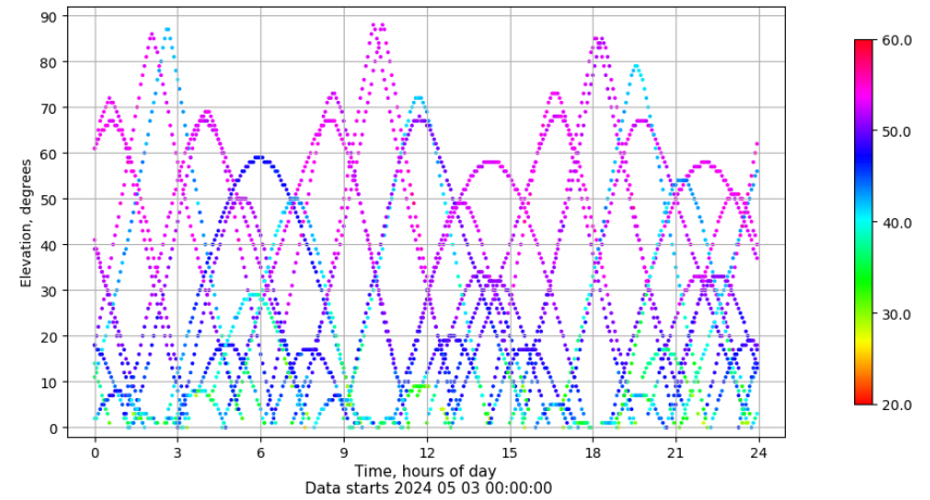
Time-elevation plot for station SALA. Signal to Noise S1C Data file SALA00ESP_R_2024124.xtr
