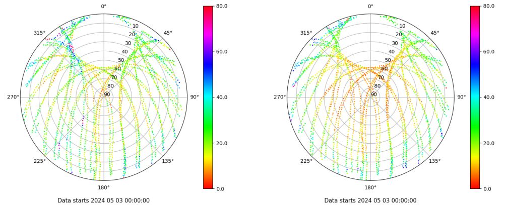
Skyplot for station SALA. Parameter M1C Data file SALA00ESP_R_2024124.xtr Skyplot for station SALA. Parameter M2P Data file SALA00ESP_R_2024124.xtr
