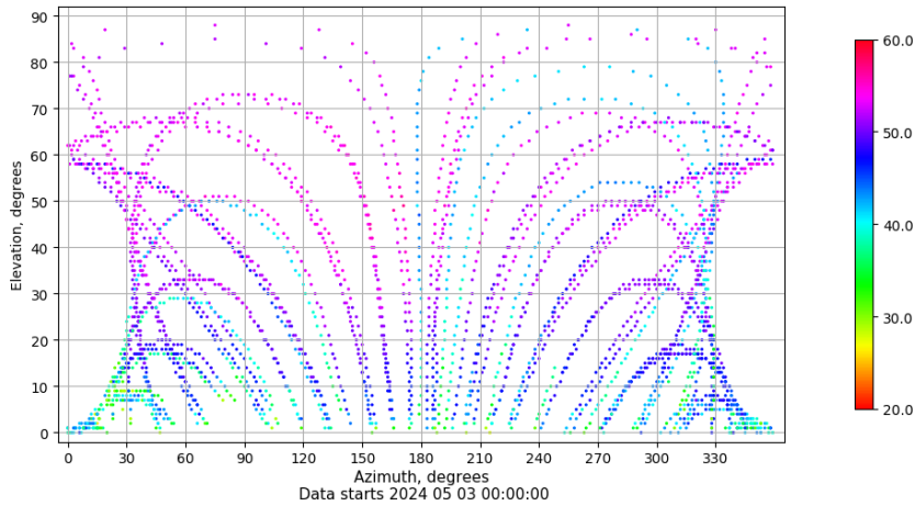
Azimuth-elevation plot for station SALA. Signal to Noise S1C Data file SALA00ESP_R_2024124.xtr
