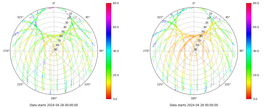
Skyplot for station SALA. Parameter M1C Data file SALA00ESP_R_2024119.xtr Skyplot for station SALA. Parameter M2P Data file SALA00ESP_R_2024119.xtr
