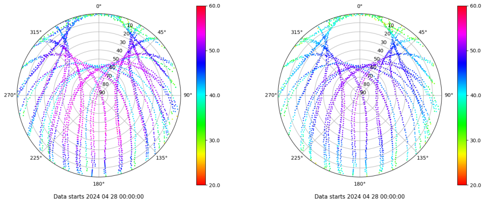
Skyplot for station SALA. Signal to Noise S1C Data file SALA00ESP_R_2024119.xtr Skyplot for station SALA. Signal to Noise S2P Data file SALA00ESP_R_2024119.xtr
