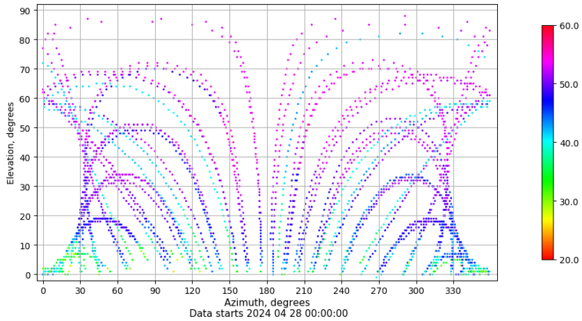
Azimuth-elevation plot for station SALA. Signal to Noise S1C Data file SALA00ESP_R_2024119.xtr
