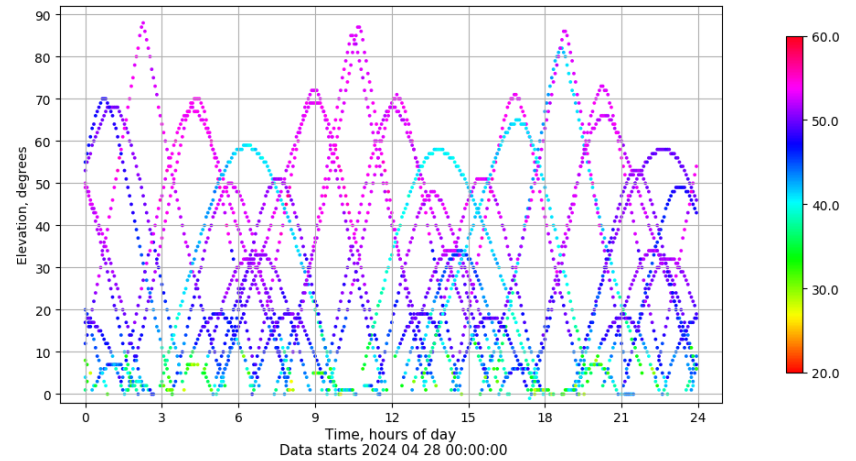
Time-elevation plot for station SALA. Signal to Noise S1C Data file SALA00ESP_R_2024119.xtr
