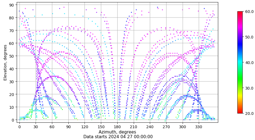
Azimuth-elevation plot for station SALA. Signal to Noise S1C Data file SALA00ESP_R_2024118.xtr
