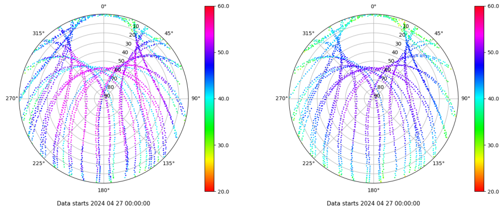
Skyplot for station SALA. Signal to Noise S1C Data file SALA00ESP_R_2024118.xtr Skyplot for station SALA. Signal to Noise S2P Data file SALA00ESP_R_2024118.xtr
