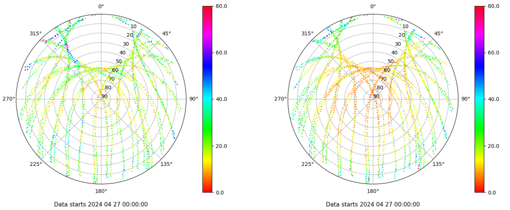
Skyplot for station SALA. Parameter M1C Data file SALA00ESP_R_2024118.xtr Skyplot for station SALA. Parameter M2P Data file SALA00ESP_R_2024118.xtr
