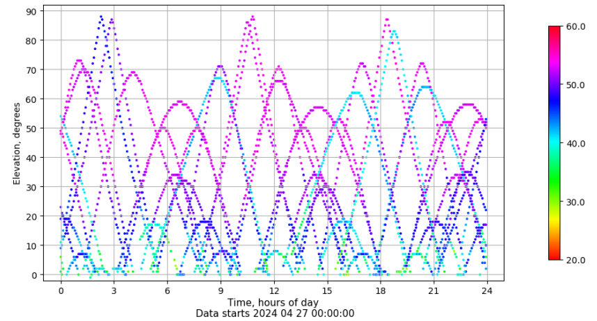
Time-elevation plot for station SALA. Signal to Noise S1C Data file SALA00ESP_R_2024118.xtr
