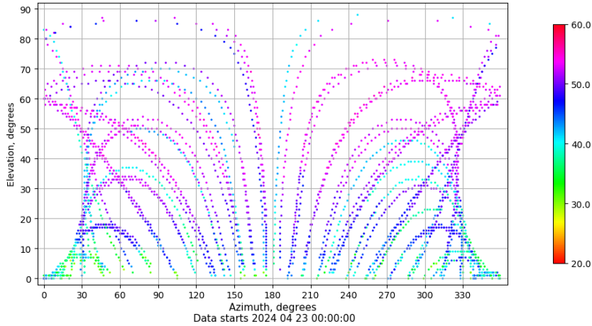
Azimuth-elevation plot for station SALA. Signal to Noise S1C Data file SALA00ESP_R_2024114.xtr
