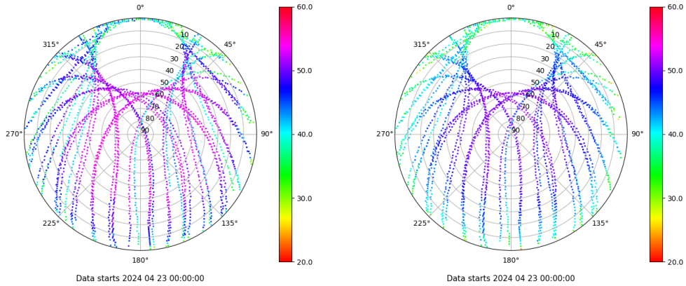
Skyplot for station SALA. Signal to Noise S1C Data file SALA00ESP_R_2024114.xtr Skyplot for station SALA. Signal to Noise S2P Data file SALA00ESP_R_2024114.xtr
