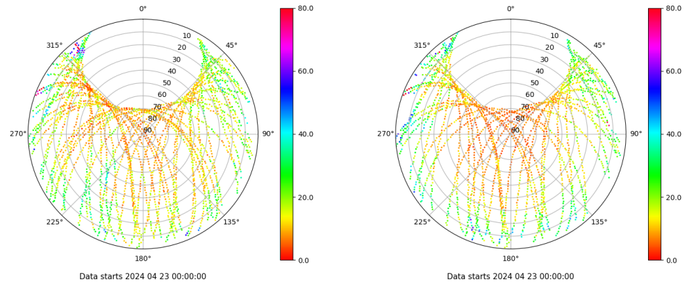
Skyplot for station SALA. Parameter M1C Data file SALA00ESP_R_2024114.xtr Skyplot for station SALA. Parameter M2S Data file SALA00ESP_R_2024114.xtr
