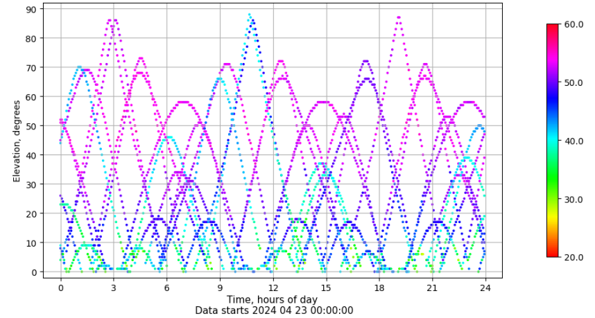
Time-elevation plot for station SALA. Signal to Noise S1C Data file SALA00ESP_R_2024114.xtr
