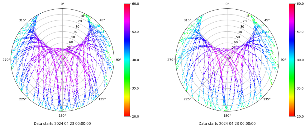
Skyplot for station SALA. Signal to Noise S1C Data file SALA00ESP_R_2024114.xtr Skyplot for station SALA. Signal to Noise S2S Data file SALA00ESP_R_2024114.xtr
