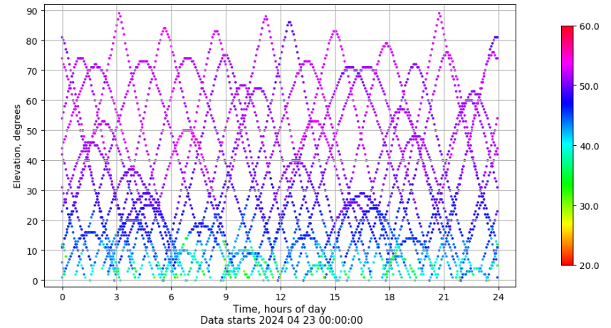
Time-elevation plot for station SALA. Signal to Noise S1C Data file SALA00ESP_R_2024114.xtr
