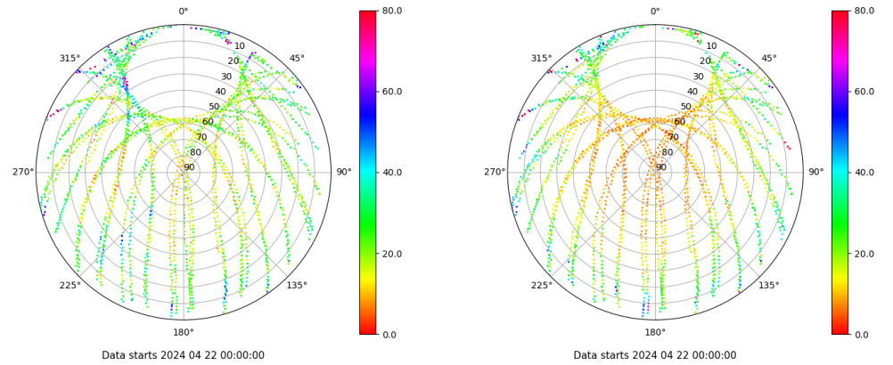
Skyplot for station SALA. Parameter M1C Data file SALA00ESP_R_2024113.xtr Skyplot for station SALA. Parameter M2P Data file SALA00ESP_R_2024113.xtr
