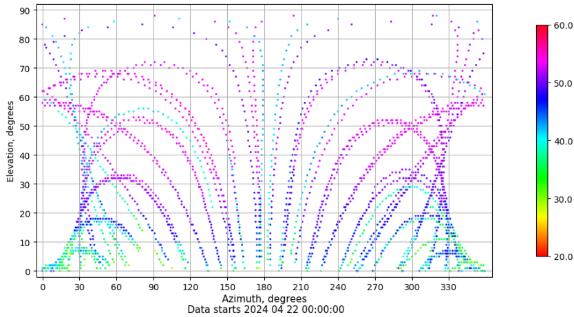
Azimuth-elevation plot for station SALA. Signal to Noise S1C Data file SALA00ESP_R_2024113.xtr
