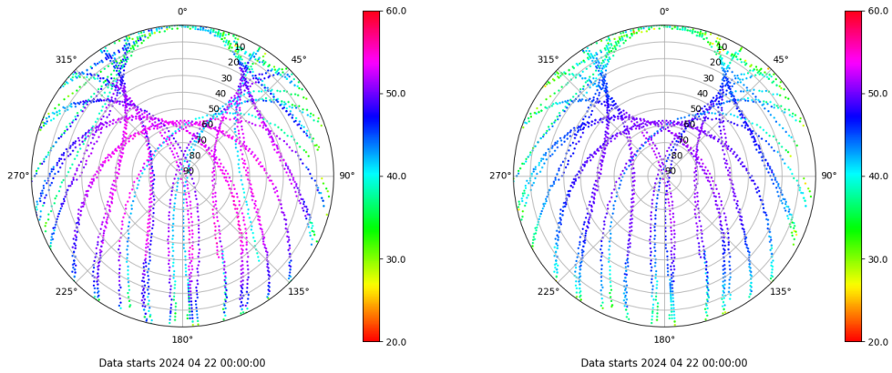
Skyplot for station SALA. Signal to Noise S1C Data file SALA00ESP_R_2024113.xtr Skyplot for station SALA. Signal to Noise S2P Data file SALA00ESP_R_2024113.xtr
