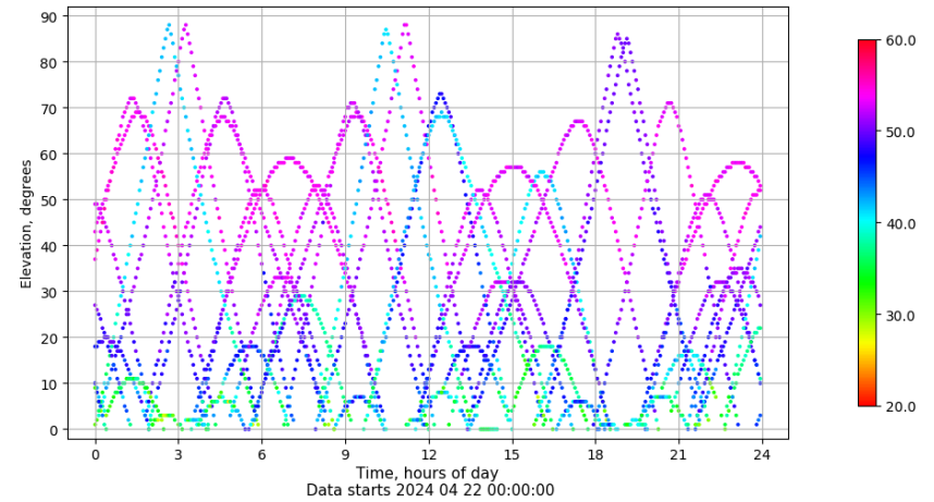
Time-elevation plot for station SALA. Signal to Noise S1C Data file SALA00ESP_R_2024113.xtr
