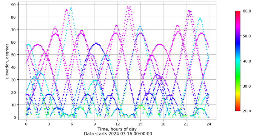
Time-elevation plot for station SALA. Signal to Noise S1C Data file SALA00ESP_R_2024076.xtr
