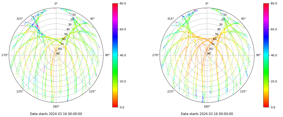
Skyplot for station SALA. Parameter M1C Data file SALA00ESP_R_2024076.xtr Skyplot for station SALA. Parameter M2P Data file SALA00ESP_R_2024076.xtr
