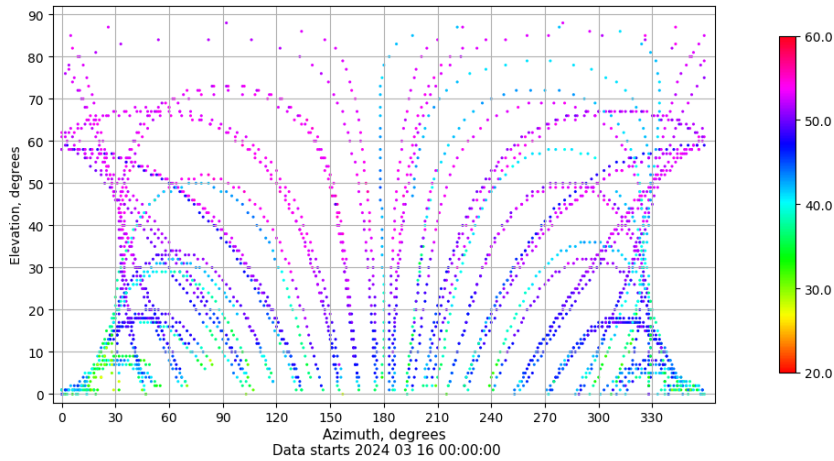
Azimuth-elevation plot for station SALA. Signal to Noise S1C Data file SALA00ESP_R_2024076.xtr
