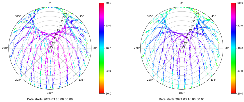
Skyplot for station SALA. Signal to Noise S1C Data file SALA00ESP_R_2024076.xtr Skyplot for station SALA. Signal to Noise S2P Data file SALA00ESP_R_2024076.xtr
