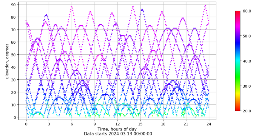
Time-elevation plot for station SALA. Signal to Noise S1C Data file SALA00ESP_R_2024073.xtr
