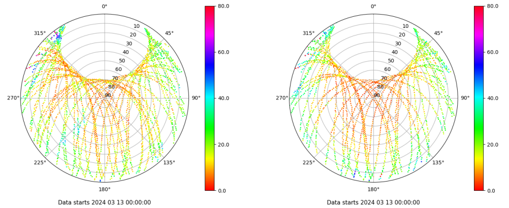
Skyplot for station SALA. Parameter M1C Data file SALA00ESP_R_2024073.xtr Skyplot for station SALA. Parameter M2S Data file SALA00ESP_R_2024073.xtr
