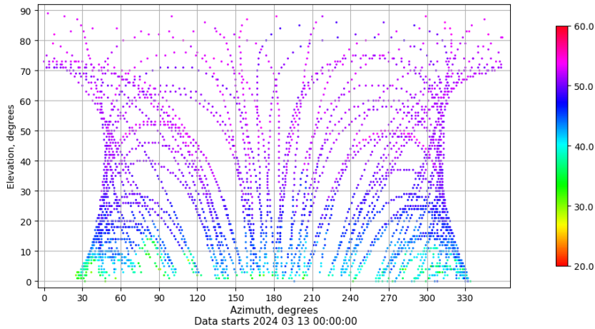
Azimuth-elevation plot for station SALA. Signal to Noise S1C Data file SALA00ESP_R_2024073.xtr
