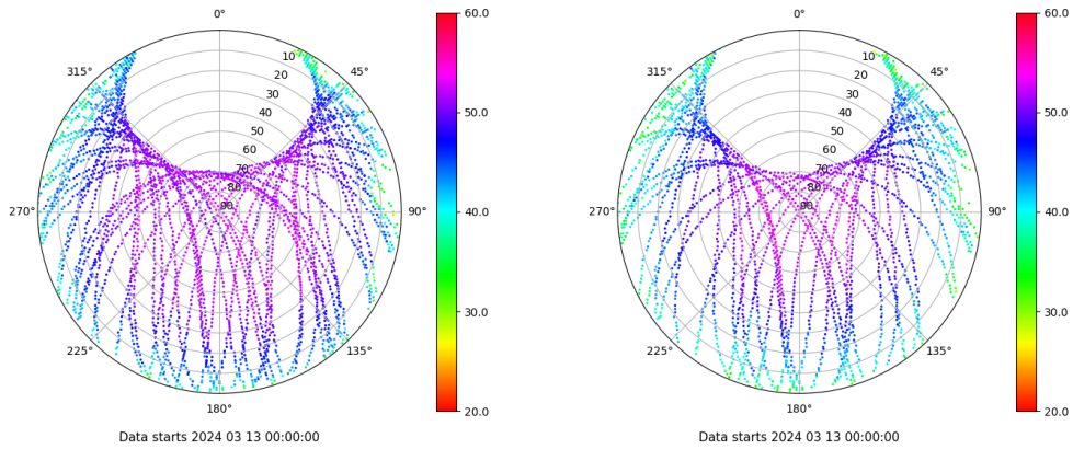
Skyplot for station SALA. Signal to Noise S1C Data file SALA00ESP_R_2024073.xtr Skyplot for station SALA. Signal to Noise S2S Data file SALA00ESP_R_2024073.xtr
