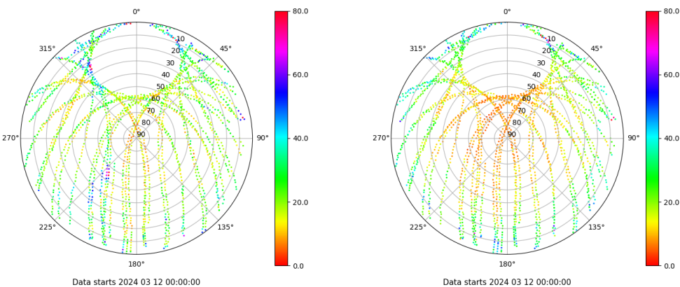
Skyplot for station SALA. Parameter M1C Data file SALA00ESP_R_2024072.xtr Skyplot for station SALA. Parameter M2P Data file SALA00ESP_R_2024072.xtr
