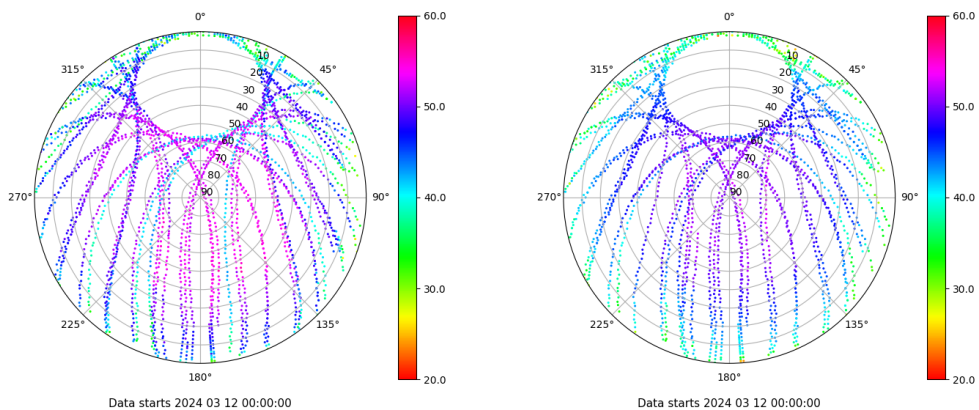
Skyplot for station SALA. Signal to Noise S1C Data file SALA00ESP_R_2024072.xtr Skyplot for station SALA. Signal to Noise S2P Data file SALA00ESP_R_2024072.xtr
