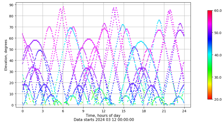
Time-elevation plot for station SALA. Signal to Noise S1C Data file SALA00ESP_R_2024072.xtr
