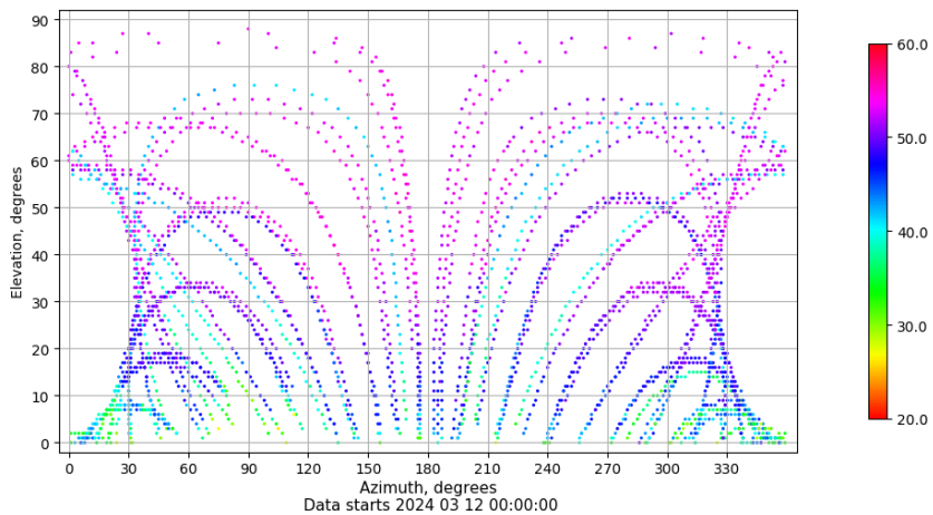
Azimuth-elevation plot for station SALA. Signal to Noise S1C Data file SALA00ESP_R_2024072.xtr
