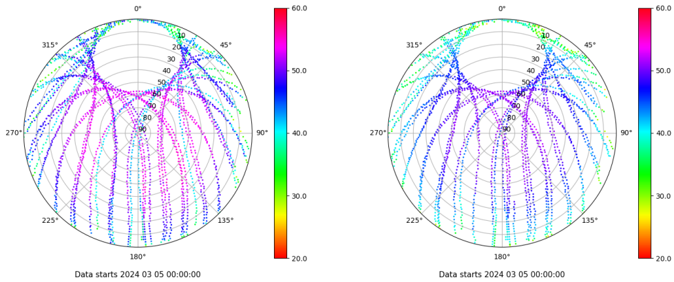
Skyplot for station SALA. Signal to Noise S1C Data file SALA00ESP_R_2024065.xtr Skyplot for station SALA. Signal to Noise S2P Data file SALA00ESP_R_2024065.xtr
