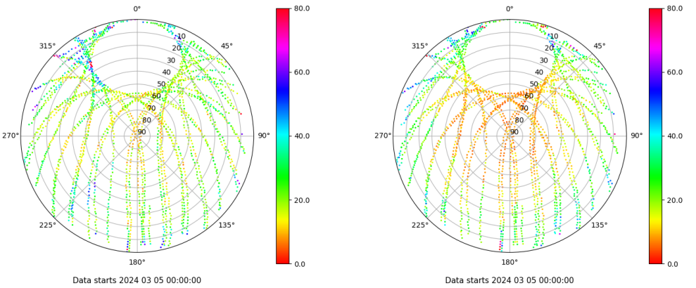
Skyplot for station SALA. Parameter M1C Data file SALA00ESP_R_2024065.xtr Skyplot for station SALA. Parameter M2P Data file SALA00ESP_R_2024065.xtr
