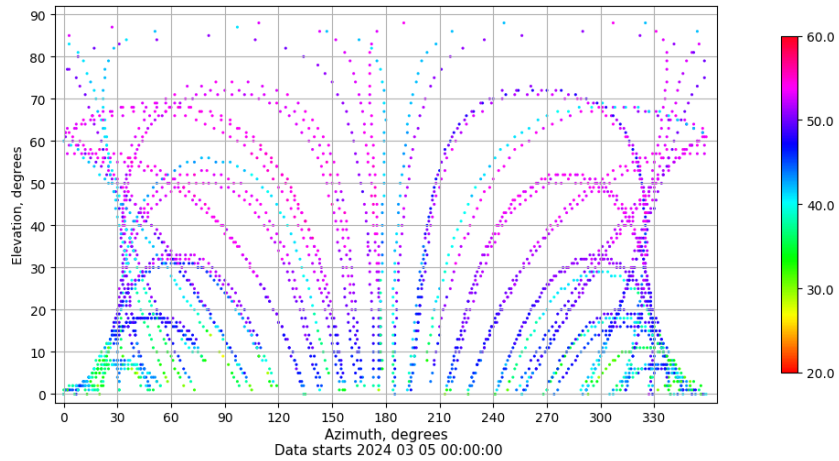
Azimuth-elevation plot for station SALA. Signal to Noise S1C Data file SALA00ESP_R_2024065.xtr
