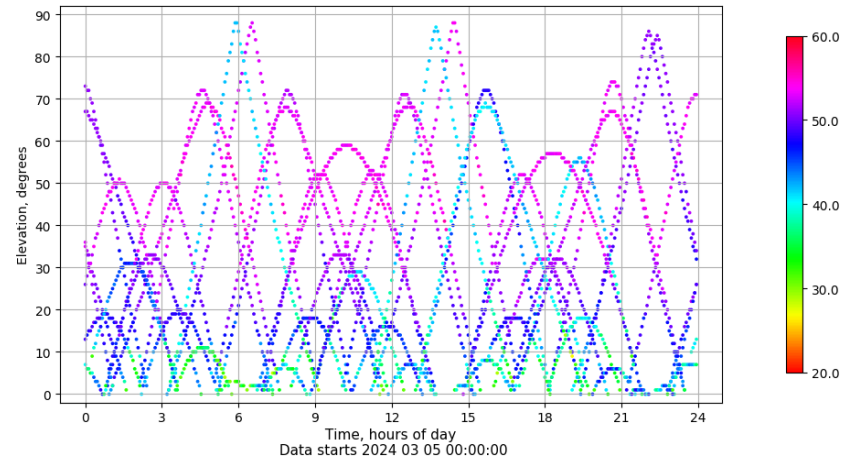
Time-elevation plot for station SALA. Signal to Noise S1C Data file SALA00ESP_R_2024065.xtr
