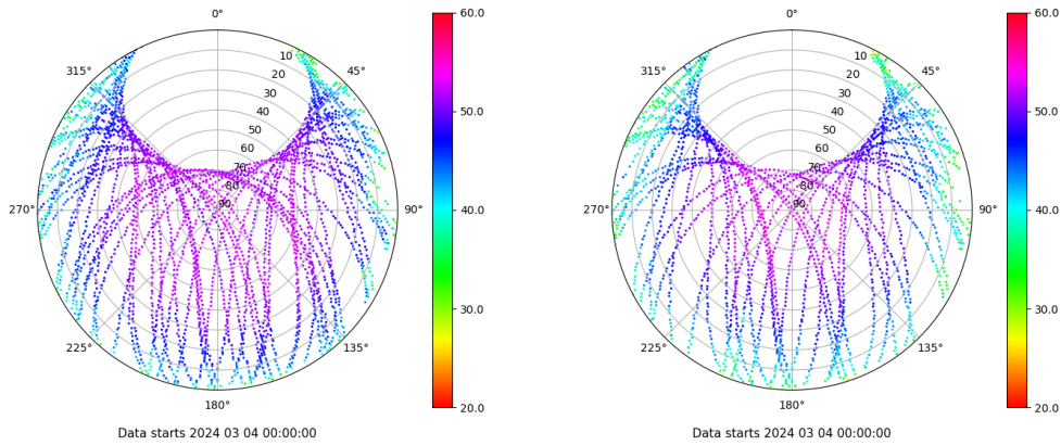
Skyplot for station SALA. Signal to Noise S1C Data file SALA00ESP_R_2024064.xtr Skyplot for station SALA. Signal to Noise S2S Data file SALA00ESP_R_2024064.xtr
