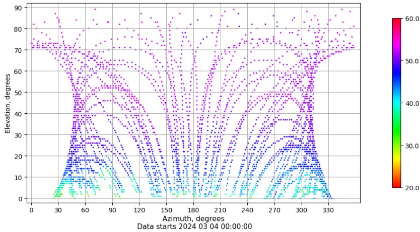
Azimuth-elevation plot for station SALA. Signal to Noise S1C Data file SALA00ESP_R_2024064.xtr
