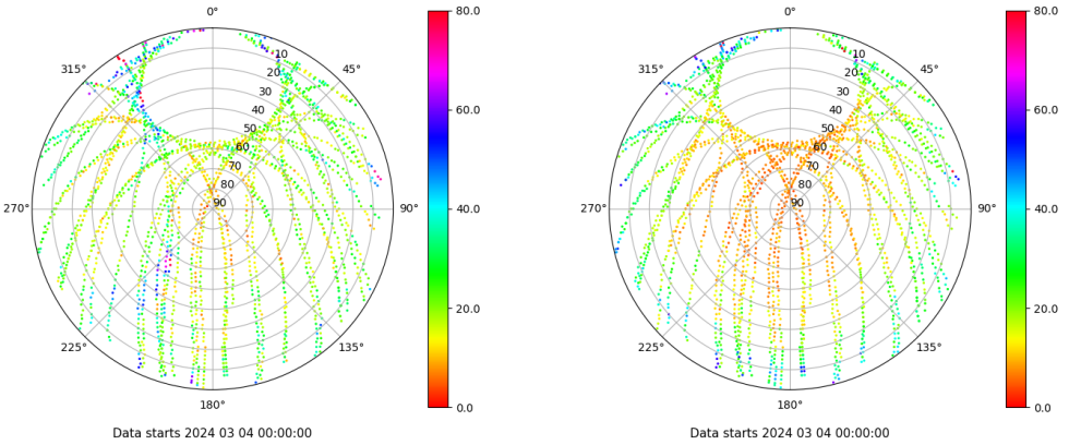
Skyplot for station SALA. Parameter M1C Data file SALA00ESP_R_2024064.xtr Skyplot for station SALA. Parameter M2P Data file SALA00ESP_R_2024064.xtr
