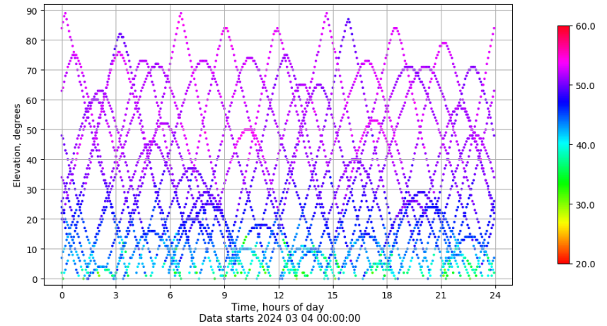
Time-elevation plot for station SALA. Signal to Noise S1C Data file SALA00ESP_R_2024064.xtr
