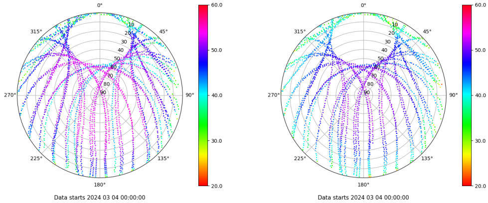
Skyplot for station SALA. Signal to Noise S1C Data file SALA00ESP_R_2024064.xtr Skyplot for station SALA. Signal to Noise S2P Data file SALA00ESP_R_2024064.xtr
