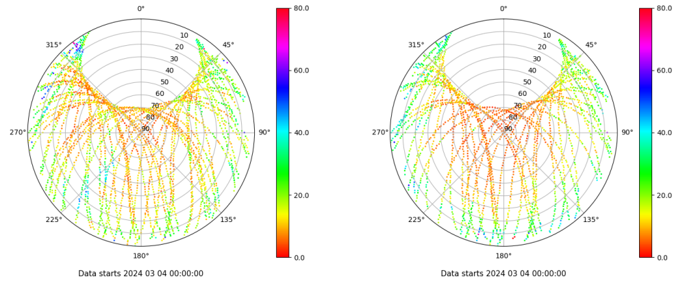
Skyplot for station SALA. Parameter M1C Data file SALA00ESP_R_2024064.xtr Skyplot for station SALA. Parameter M2S Data file SALA00ESP_R_2024064.xtr
