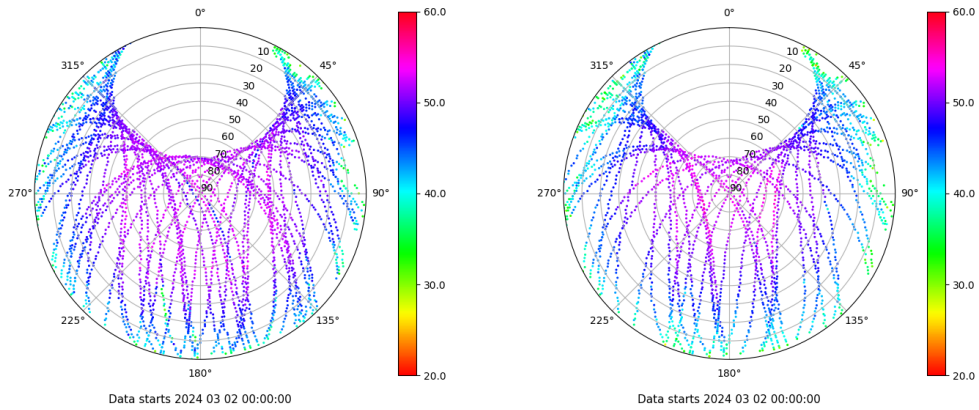
Skyplot for station SALA. Signal to Noise S1C Data file SALA00ESP_R_2024062.xtr Skyplot for station SALA. Signal to Noise S2S Data file SALA00ESP_R_2024062.xtr
