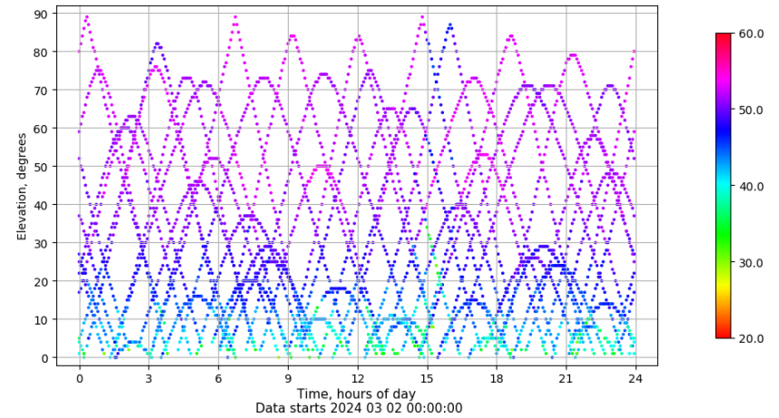
Time-elevation plot for station SALA. Signal to Noise S1C Data file SALA00ESP_R_2024062.xtr
