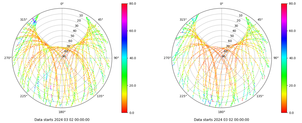
Skyplot for station SALA. Parameter M1C Data file SALA00ESP_R_2024062.xtr Skyplot for station SALA. Parameter M2S Data file SALA00ESP_R_2024062.xtr
