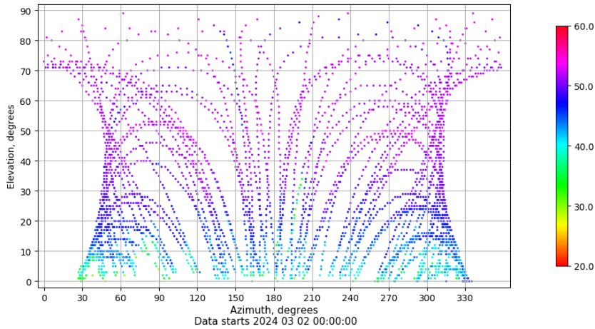
Azimuth-elevation plot for station SALA. Signal to Noise S1C Data file SALA00ESP_R_2024062.xtr
