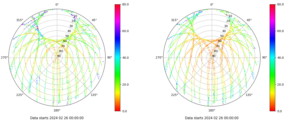
Skyplot for station SALA. Parameter M1C Data file SALA00ESP_R_2024057.xtr Skyplot for station SALA. Parameter M2P Data file SALA00ESP_R_2024057.xtr
