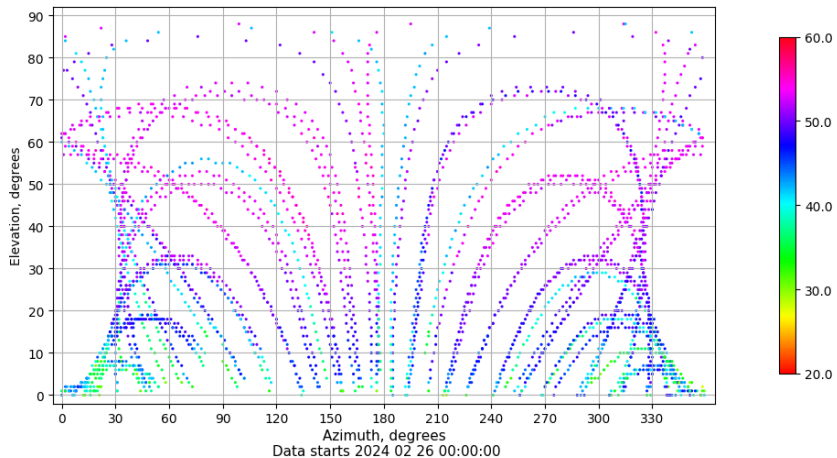
Azimuth-elevation plot for station SALA. Signal to Noise S1C Data file SALA00ESP_R_2024057.xtr
