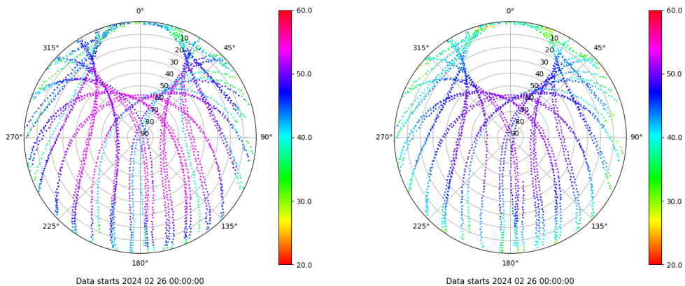
Skyplot for station SALA. Signal to Noise S1C Data file SALA00ESP_R_2024057.xtr Skyplot for station SALA. Signal to Noise S2P Data file SALA00ESP_R_2024057.xtr
