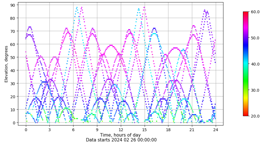
Time-elevation plot for station SALA. Signal to Noise S1C Data file SALA00ESP_R_2024057.xtr
