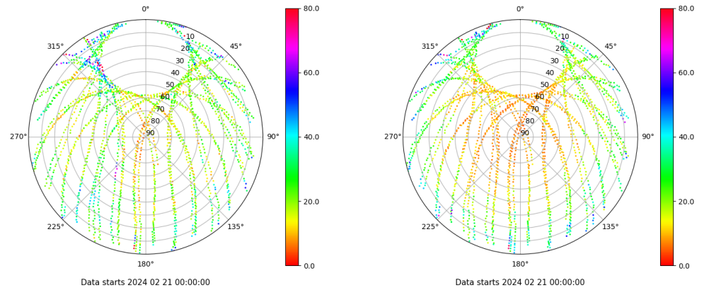
Skyplot for station SALA. Parameter M1C Data file SALA00ESP_R_2024052.xtr Skyplot for station SALA. Parameter M2P Data file SALA00ESP_R_2024052.xtr
