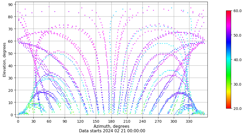
Azimuth-elevation plot for station SALA. Signal to Noise S1C Data file SALA00ESP_R_2024052.xtr
