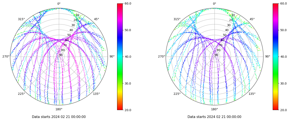
Skyplot for station SALA. Signal to Noise S1C Data file SALA00ESP_R_2024052.xtr Skyplot for station SALA. Signal to Noise S2P Data file SALA00ESP_R_2024052.xtr
