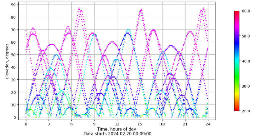
Time-elevation plot for station SALA. Signal to Noise S1C Data file SALA00ESP_R_2024051.xtr
