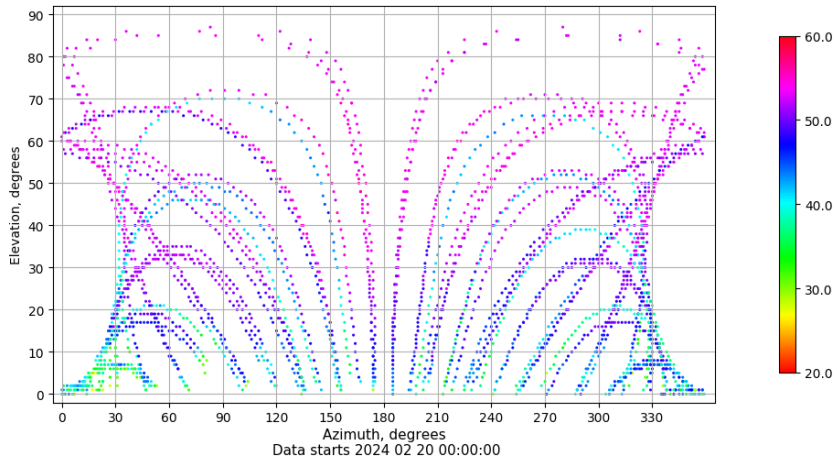
Azimuth-elevation plot for station SALA. Signal to Noise S1C Data file SALA00ESP_R_2024051.xtr
