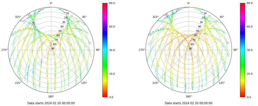
Skyplot for station SALA. Parameter M1C Data file SALA00ESP_R_2024051.xtr Skyplot for station SALA. Parameter M2P Data file SALA00ESP_R_2024051.xtr
