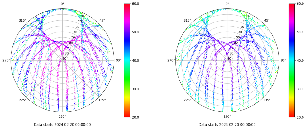
Skyplot for station SALA. Signal to Noise S1C Data file SALA00ESP_R_2024051.xtr Skyplot for station SALA. Signal to Noise S2P Data file SALA00ESP_R_2024051.xtr
