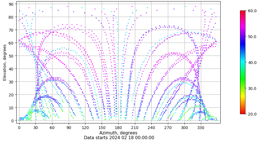
Azimuth-elevation plot for station SALA. Signal to Noise S1C Data file SALA00ESP_R_2024049.xtr
