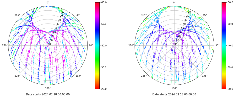
Skyplot for station SALA. Signal to Noise S1C Data file SALA00ESP_R_2024049.xtr Skyplot for station SALA. Signal to Noise S2P Data file SALA00ESP_R_2024049.xtr
