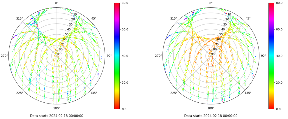
Skyplot for station SALA. Parameter M1C Data file SALA00ESP_R_2024049.xtr Skyplot for station SALA. Parameter M2P Data file SALA00ESP_R_2024049.xtr
