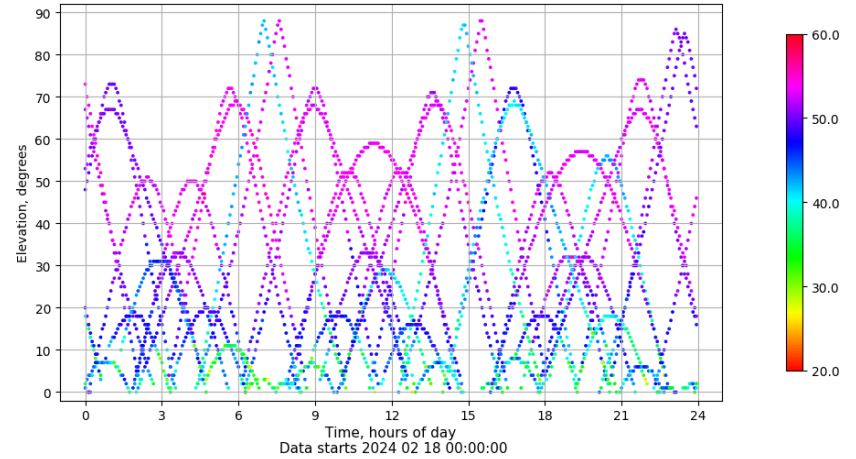
Time-elevation plot for station SALA. Signal to Noise S1C Data file SALA00ESP_R_2024049.xtr
